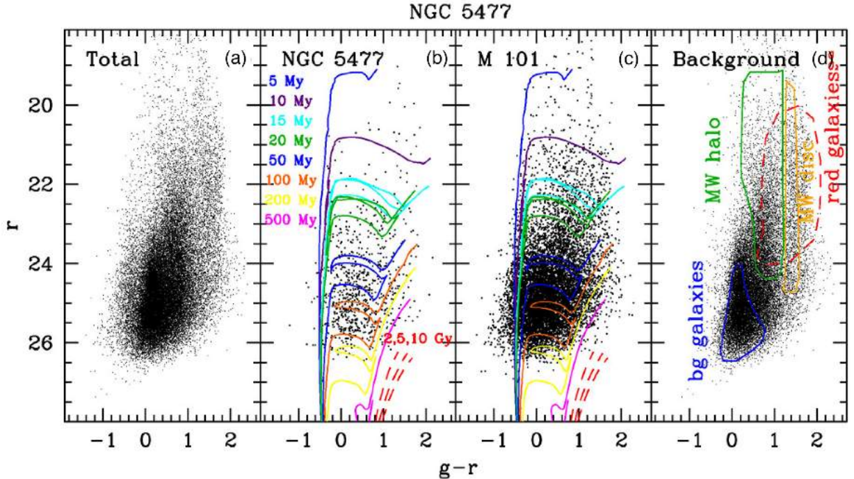
Figure 11. r, g-r CMD of NGC 5477. (a): Total CMD over the whole 23 arcmin \times 23 arcmin LBC field of view. (b): CMD of stars within an elliptical region of SMA = 2 arcmin centred on NGC 5477; overplotted are the PARSEC isochrones shifted to a distance of D = 6.8 Mpc [ (m - M)_0 = 29.2 ] and corrected for a foreground reddening of E(B - V) = 0.01 . The isochrones' metallicity of Z = 0.002 is consistent with the H II region oxygen abundance of 12 + \log(\text{O}/\text{H}) = 7.9 (Berg et al. 2012). (c): CMD of a region including the spiral galaxy M 101, according to the contour displayed in Fig. 5. (d): CMD of stars outside the regions including NGC 5477 and M 101, mostly sampling background galaxies, and foreground MW halo and disc stars, as labelled in the plot.
