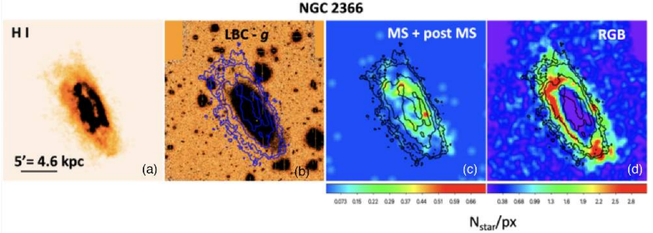
Figure 14. Panel (a): H I emission image of NGC 2366 from LITTLE THINGS (Hunter et al. 2012). Panel (b): LBC image in g with superimposed the H I contours for mass densities of \sim 0.6, 1.8, 5.4 , and 16.2 \text{ M}_{\odot} \text{ pc}^{-2} (see Iorio et al. 2017). Panel (c): density map of blue MS and post MS stars with age \lesssim 200 \text{ Myr} selected within the box outlined in Fig. 8; the scale is in number of stars per pixel, where the pixel size is \sim 10 \text{ arcsec} \times 10 \text{ arcsec} . Superimposed are the H I contours. Panel (d): Same as (c) but for RGB stars, with ages > 1\text{--}2 \text{ Gyr} . All four images are displayed on the same spatial scale, with a field of view of \sim 23 \text{ arcmin} \times 23 \text{ arcmin} .
