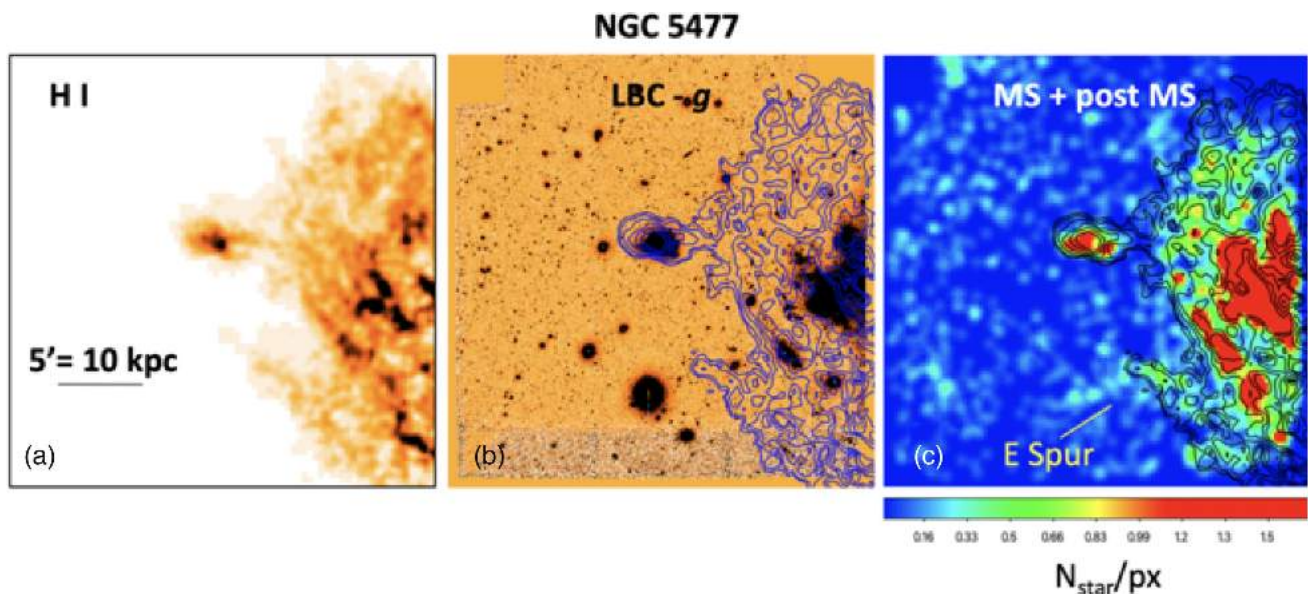
Figure 16. Panel (a): H I emission image of NGC 5477 from WHISP (Swaters et al. 2002). Panel (b): LBC image in g with superimposed the H I contours for mass densities of \sim 1, 3, 4, 5, 8 , and 11 \text{ M}_{\odot} \text{ pc}^{-2} . Panel (c): density map of young (age \lesssim 100 \text{ Myr} ) MS and post-MS stars in number of stars per pixel (pixel size = 10 \text{ arcsec} \times 10 \text{ arcsec} ) selected from the CMD of NGC 5477 (see Fig. 11); superimposed are the H I contours. On the density map, we indicate the E Spur identified by Mihos et al. (2013) from deep optical images. All three images are displayed on the same spatial scale, with a field of view of \sim 25 \text{ arcmin} \times 24 \text{ arcmin} .
