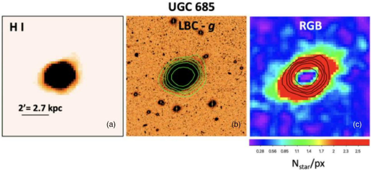
Figure 15. Panel (a): H I emission image of UGC 685 from the FIGGS survey (Begum et al. 2008), kindly provided by S. Roychowdhury. Panel (b): LBC image in g with superimposed the H I contours for mass densities of \sim 0.1, 0.5, 1, 2 , and 5 \text{ M}_{\odot} \text{ pc}^{-2} . Panel (c): Density map of RGB stars in counts per pixel (pixel size = 10 \text{ arcsec} \times 10 \text{ arcsec} ) with superimposed the H I contours. All four images are displayed on the same spatial scale, with a field of view of \sim 9 \text{ arcmin} \times 9 \text{ arcmin} .
