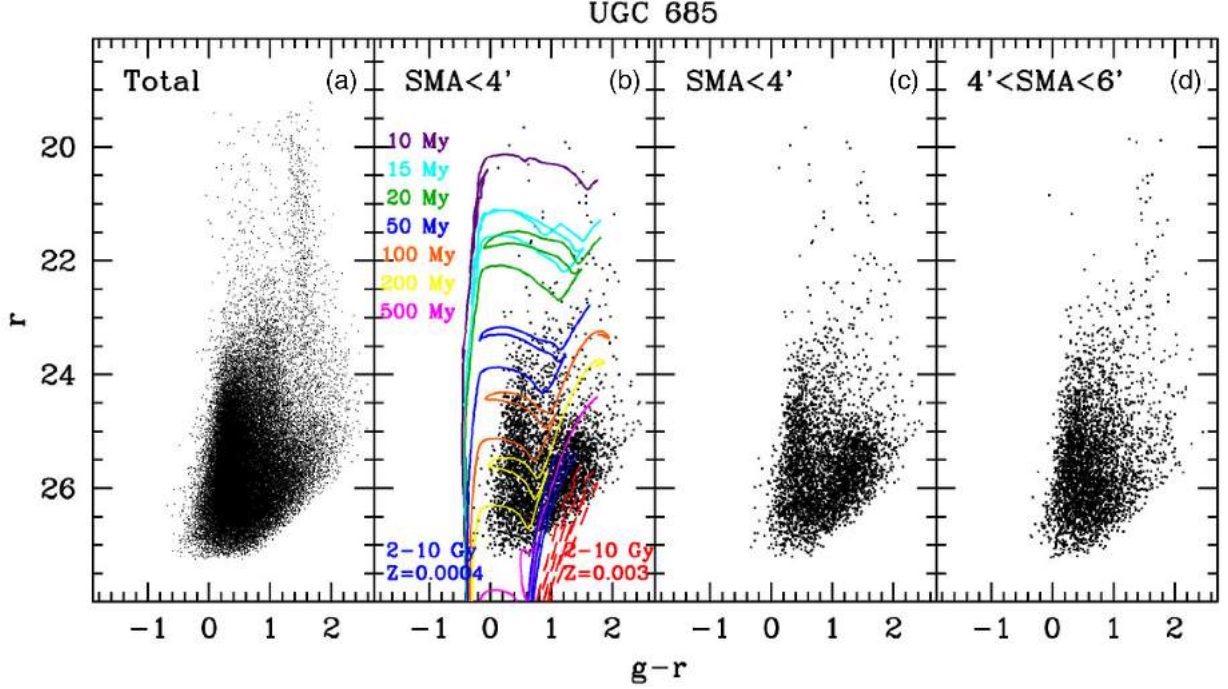
Figure 10. r, g-r CMD of UGC 685. (a): Total CMD over the whole 23 arcmin \times 23 arcmin LBC field of view. (b): CMD of stars within an elliptical region of SMA = 4 arcmin, with overplotted the PARSEC isochrones shifted to a distance of D = 4.7 Mpc [ (m - M)_0 = 28.4 ] and corrected for a foreground reddening of E(B - V) = 0.05 . The displayed isochrones have a metallicity of Z = 0.003 , compatible with the H II regions metallicity of 12 + \log(\text{O}/\text{H}) = 8.00 (van Zee & Haynes 2006). For ages \geq 2 Gyr, we also show the Z = 0.0004 ( \sim 1/40 solar) metallicity models. (c): Same as (b), but with no models superimposed. (d) CMD of stars in an adjacent external field at 4 arcmin < \text{SMA} < 6 arcmin, containing approximately the same number of stars as (b), and mostly sampling background galaxies and MW foreground stars.
