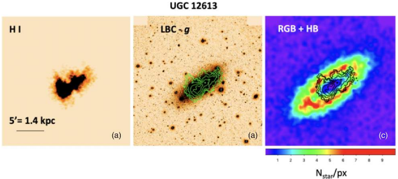
Figure 13. Panel (a): H I emission image of UGC 12613 from LITTLE THINGS (Hunter et al. 2012). Panel (b): LBC image in g with superimposed the H I contours for mass densities of \sim 0.4, 0.8, 1.6 , and 3.2 \text{ M}_\odot \text{ pc}^{-2} (see Iorio et al. 2017). Panel (c): density map of RGB plus HB/RC stars in number of stars per pixel (where the pixel size is \sim 10 \text{ arcsec} \times 10 \text{ arcsec} ) selected from the CMD of UGC 12613 (see Fig. 6); superimposed are the H I contours. All three images are displayed on the same spatial scale, with a field of view of \sim 23.5 \text{ arcmin} \times 23.5 \text{ arcmin} .
