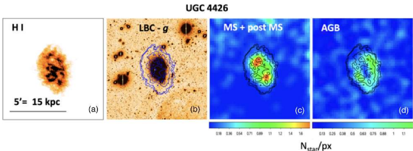
Figure 17. Panel (a): H I emission image of UGC 4426 from LITTLE THINGS (Hunter et al. 2012). Panel (b): LBC image in g with superimposed the H I contours for mass densities of \sim 0.5, 1, 3 , and 5 \text{ M}_{\odot} \text{ pc}^{-2} . Panel (c): density map of young (age \lesssim 100 \text{ Myr} ) MS and post-MS stars in number of stars per pixel (where the pixel size is 10 \text{ arcsec} \times 10 \text{ arcsec} ) selected from the CMD of UGC 4426 (see Fig. 12); superimposed are the H I contours. Panel (d): density map of sources with g - r \gtrsim 1, r \gtrsim 26 , which are AGB stars with age > 500 \text{ Myr} or blends of two or more fainter RGB stars. All three images are displayed on the same spatial scale, with a field of view of \sim 9 \text{ arcmin} \times 9 \text{ arcmin} .
