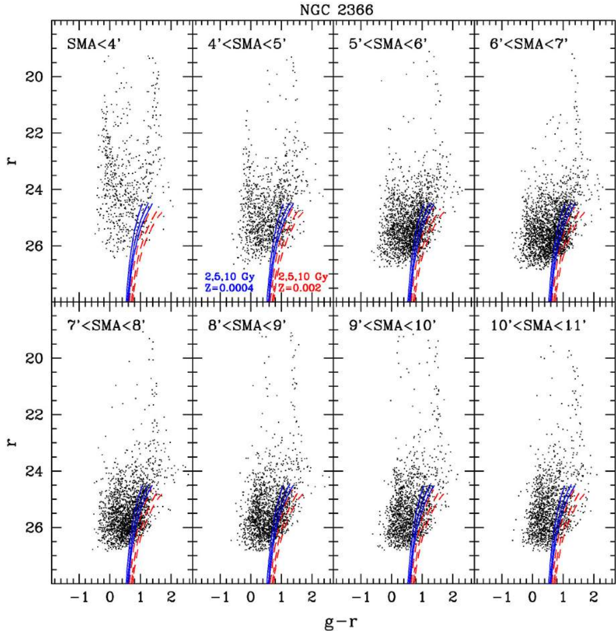
Figure 9. CMDs of NGC 2366 selected in elliptical annuli of increasing SMA. Overplotted are the RGB portions of the PARSEC (Bressan et al. 2012) isochrones in the SDSS photometric system shifted to a distance of D = 3.2 Mpc ( (m - M)_0 = 27.5 ). The dotted (red in the electronic version of the paper) isochrones have metallicity Z = 0.002 , whilst the solid ones (blue) have Z = 0.0004 . For clarity, the thermally pulsing AGB models have not been displayed in the plot.
