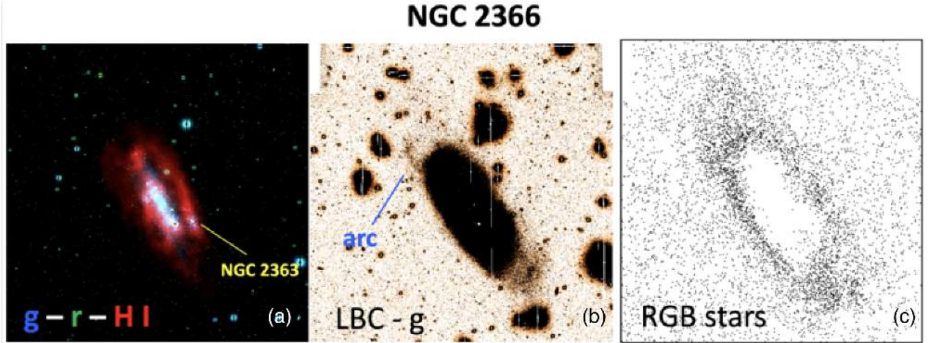
Figure 21. Panel (a): g-r -H I colour-combined image of NGC 2366 highlighting the presence of two parallel ridges of H I that appear to connect NGC 2366 to the giant H II region complex NGC 2363. Panel (b): Deep LBC g image with the display cuts chosen to emphasize a low SB arc. Panel (c): distribution of RGB stars extending out to much larger galactocentric distances than visible from the LBC image. All images have been displayed on the same spatial scale. North is up and east is left.
