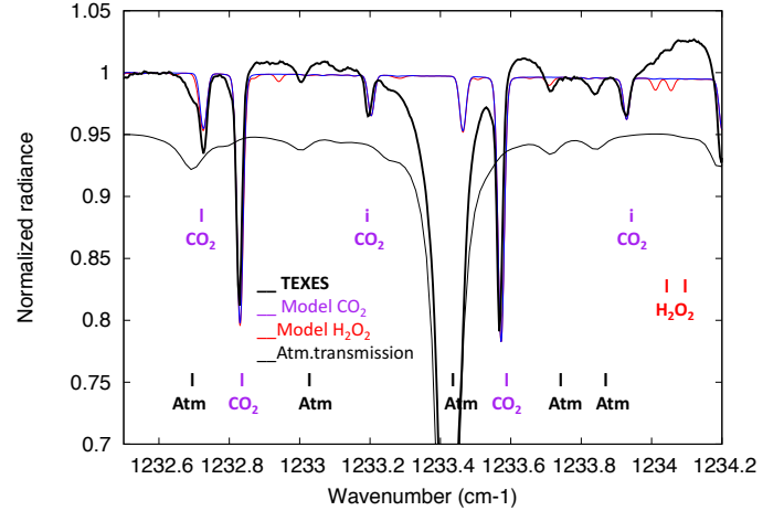
Fig. 1. Thick black line: spectrum of Mars between 1232.6 and 1234.2 \text{cm}^{-1} , integrated over the Martian disk, recorded on May 7, 2016 ( \text{Ls} = 148.5^\circ , normalized radiance). Synthetic spectra of Mars: \text{CO}_2 alone (blue), \text{H}_2\text{O}_2 alone with \text{H}_2\text{O}_2/\text{CO}_2 = 100 ppbv (red). Thin black line (in absolute units shifted by -0.05 ): transmission from the terrestrial atmosphere, as measured by the TEXES instrument. “Atm” indicates terrestrial absorption.
