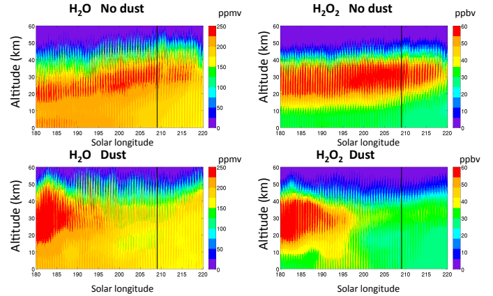
Fig. 17. Vertical distributions of H 2 O ( left ) and H 2 O 2 ( right ) as a function of the solar longitude at the beginning of southern summer (Ls = 180–220°). Top : clear conditions; bottom : dusty conditions. Simulations were done with the GEM model (Daerden et al. 2019) for the latitude of the subsolar point (12° S).
