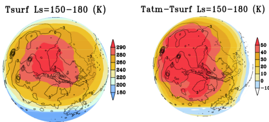
Fig. 3. Synthetic maps of (left) the surface temperature, and (right) the temperature contrast T(z=1\text{ km}) - T_s , for the seasonal range L_s = 150-180^\circ . The maps are from the Mars Climate Database (Forget et al. 1999).
