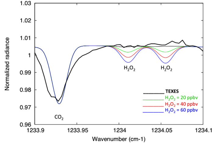
Fig. 6. Bold dark line: spectrum of Mars between 1233.9 and 1234.1 cm -1 , integrated over the southern hemisphere of the planet, recorded on May 7, 2016 (Ls = 148°, normalized radiance). Thin lines: synthetic models, calculated using the atmospheric parameters described in Sect. 2.2: Black: H 2 O 2 = 0 ppbv; green: H 2 O 2 = 20 ppbv; red: H 2 O 2 = 40 ppbv; blue: H 2 O 2 = 60 ppbv. H 2 O 2 is undetected, with a 2\sigma upper limit of 10 ppbv. The poor fit of the CO 2 line in the southern hemisphere is due to the occasional presence of a spike near the line center. The spectral resolution of the models is 0.024 cm -1 .
