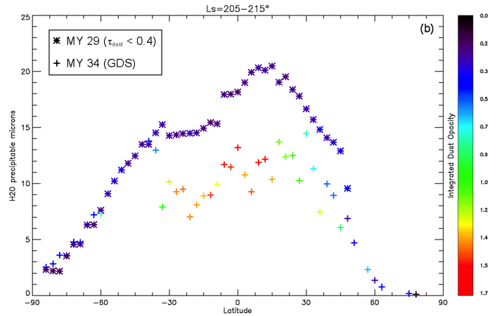
Fig. 18. Latitudinal variations in the water vapor column density observed by PFS between Ls = 205° and 215° in the case of MY 29, corresponding to a dust opacity lower than 0.4 (stars), and M34, a great dust storm (crosses). The color bar on the right of the figure indicates the integrated dust opacity. The figure is taken from Giuranna & Wolkenberg (2019).
