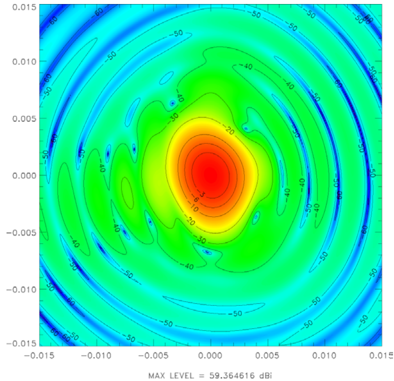
Figure 28 Co- polar component of Main Beam #21, ET 15dB@22°.
