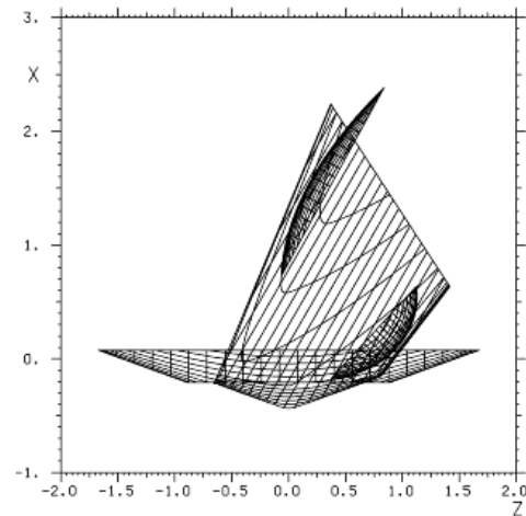
Figure 1 Planck/LFI Focal Plane Unit configuration. The 70 GHz LFI feed horns studied are marked with red circles. The axes are the X- and Y- axes of the Reference Detector Plane System (left). Telescope and shields geometry in (XZ)_{\text{TEL}} plane (right).
