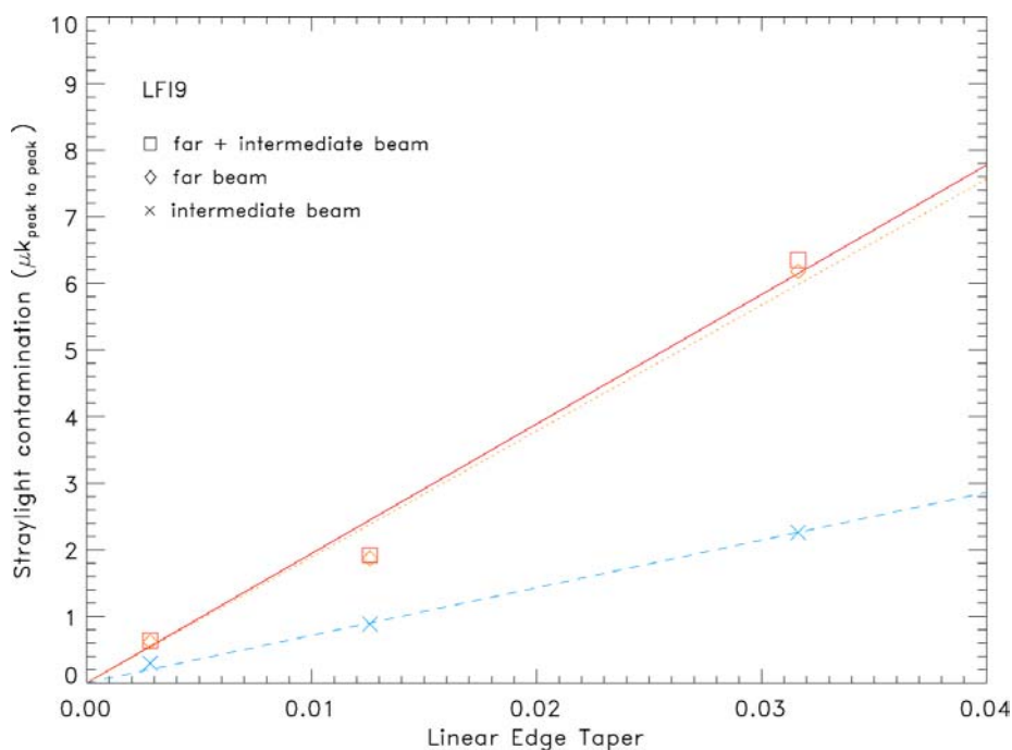
Figure 3 Correlation between Straylight Contamination ( \mu k , peak to peak) and Edge Taper for the 100 GHz LFI feed horn #9.
