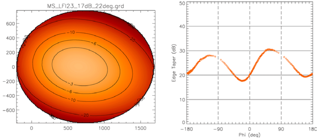
Figure 5 Field Distribution on the main reflector illuminated by the Gaussian feed #23 with an ET equal to 17dB@22°.
