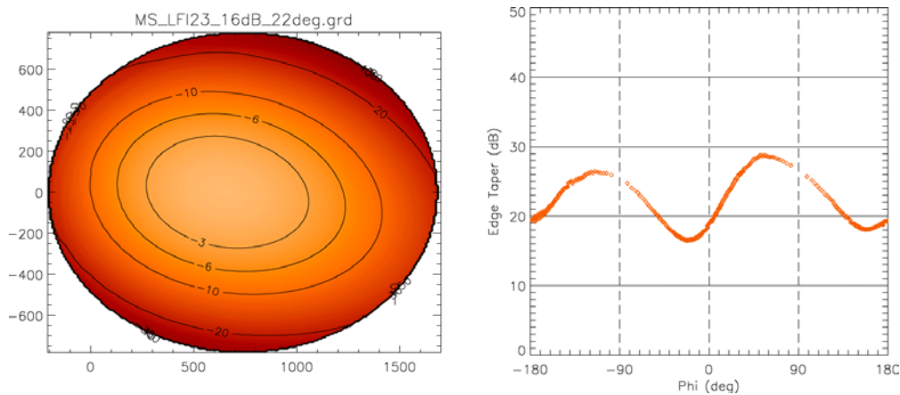
Figure 7 Field Distribution on the main reflector illuminated by the Gaussian feed #23 with an ET equal to 16dB@22°.
