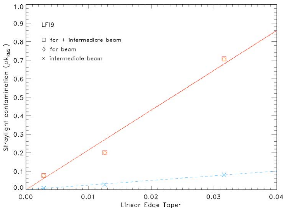
Figure 4 Correlation between Straylight Contamination ( \mu k , RMS) and Edge Taper for the 100 GHz LFI feed horn #9.
