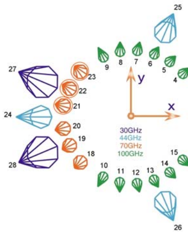
Figure 1 Planck/LFI Focal Plane Unit configuration. The 70 GHz LFI feed horns studied are marked with red circles. The axes are the X- and Y- axes of the Reference Detector Plane System (left). Telescope and shields geometry in (XZ)_{\text{TEL}} plane (right).
