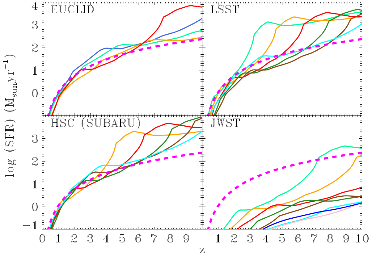
Figure 14. Minimum SFR detectable by the deepest SKA1-MID survey at 1.4 GHz (down to 0.25 \mu\text{Jy} , dashed magenta line), compared with the minimum SFR detectable in each spectral band by the Euclid deep survey, by the Subaru HSC ultra-deep survey, by the LSST deep drilling fields and by the JWST DWS for the obscured SED shown in the right panel of Figure 15.
