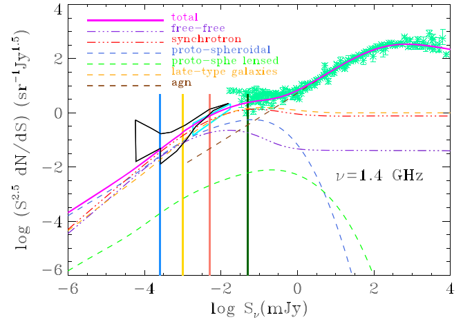
Figure 3. Euclidean normalized differential counts at 1.4 GHz compared with model predictions. Above \sim 1 mJy the counts are dominated by canonical radio-loud active galactic nuclei (AGNs) while star-forming galaxies take over at fainter flux densities. The dashed brown line shows the model for radio AGNs by Massardi et al. (2010). The other dashed lines show the contributions of the star-forming populations considered in this paper (unlensed and strongly lensed proto-spheroids and late-type galaxies). The two triple-dot-dashed lines show the total synchrotron and free-free emissions from these populations. References for the data points can be found in de Zotti et al. (2010). The cyan and the black polygons show the ranges of 1.4 GHz counts consistent with the P(D) distributions by Condon et al. (2012) and Vernstrom et al. (2014), respectively. Note that these P(D) analyses rule out the sub-mJy counts as high as the Owen & Morrison (2008) estimates. As argued by Condon et al. (2012) the high counts may result from the large and difficult corrections for the effects of partial resolution; the quoted P(D) data do not need significant resolution corrections. The vertical lines correspond, from left to right, to the 5\sigma detection limits of the planned SKA1-MID surveys to unresolved sources: 0.25 \mu\text{Jy} (blue), 1 \mu\text{Jy} (yellow), 5 \mu\text{Jy} (pink). Given the resolution of these surveys ( \approx 0''.5 ; Prandoni & Seymour 2014) it is likely that a fraction of sources (especially bright, nearby galaxies) will be resolved out so that the surveys will not be 100% complete at the quoted limits. However, the array configuration proposed, which delivers an essentially flat point source sensitivity over a large range of synthesized beams, will overcome this problem. The 5 \mu\text{Jy} limit applies also to the Tier 2 MIGHTEE survey (MeerKAT), while the dark green line shows the EMU (ASKAP) survey 5\sigma limit. Again, the limits refer to unresolved sources. The MIGHTEE and EMU surveys have a lower resolution than the SKA1-MID ones: 8''.3 – 3''.5 in the case of Tier 2 MIGHTEE ( http://www.ast.ucl.ac.za/arniston2011/vdheyden.pdf ) and 10'' in the case of EMU (Norris et al. 2011).
