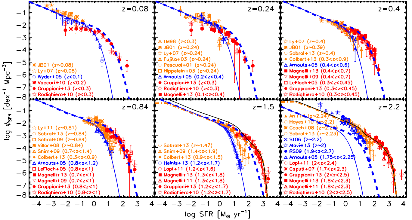
Figure 1. SFR functions at several redshifts. The blue lines show the SFR functions derived from the UV luminosity functions given by the phenomenological model for late-type galaxies with and without the extinction correction (dashed and thin solid lines, respectively). The dot-dashed orange lines show the contributions given by the physical model for proto-spheroids with a minimum halo mass M_{\text{vir}}^{\text{min}} = 10^{8.5} M_{\odot} . The thick black lines show the sum of the contributions from late-type galaxies, after the extinction correction, and of proto-spheroids. The red data points are estimates from far-IR measurements (Caputi et al. 2007; Rodighiero et al. 2010; Lapi et al. 2011; Magnelli et al. 2011, 2013; Gruppioni et al. 2013). The blue data points are from UV measurements (Steidel et al. 1999; Arnouts et al. 2005; Wyder et al. 2005; Sawicki & Thompson 2006; Reddy & Steidel 2009; Heinis et al. 2013; Alavi et al. 2014). The orange data points are from H \alpha measurements (Tresse & Maddox 1998; Jones & Bland-Hawthorn 2001; Pascual et al. 2001; Fujita et al. 2003; Hippelein et al. 2003; Ly et al. 2007, 2012; Geach et al. 2008; Villar et al. 2008; Sobral et al. 2009, 2013; Hayes et al. 2010). The conversions of attenuated UV and H \alpha luminosities to SFRs are done using the Kennicutt & Evans (2012) calibrations, i.e., \log(\text{SFR}/[M_{\odot} \text{ yr}^{-1}]) = \log(L_{\text{FUV}}/[L_{\odot}]) - 9.825 and \log(\text{SFR}/[M_{\odot} \text{ yr}^{-1}]) = \log(L_{\text{H}\alpha}/[\text{erg s}^{-1}]) - 41.270 , respectively. The conversion of the IR luminosity to SFR was done using Equation (1), which takes into account that a substantial contribution to dust heating in galaxies with low SFRs comes from old stellar populations. Comparing the SFRs estimated from the UV or from the H \alpha luminosities with those inferred from the IR luminosities it is apparent that the former are increasingly underestimated with increasing SFR and redshift, consistent with the findings by Reddy et al. (2012) and Burgarella et al. (2013).
