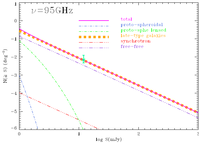
Figure 6. Our reassessment of the integral counts of dusty galaxies at \nu = 95 GHz (asterisks with error bars) compared with the expectations from the Cai et al. (2013) model, using for each source populations the complete SEDs that include dust, synchrotron, and free-free emissions. The various lines correspond to the contributions from the different source populations and from the different emission processes, identified in the legend inside the figure.
