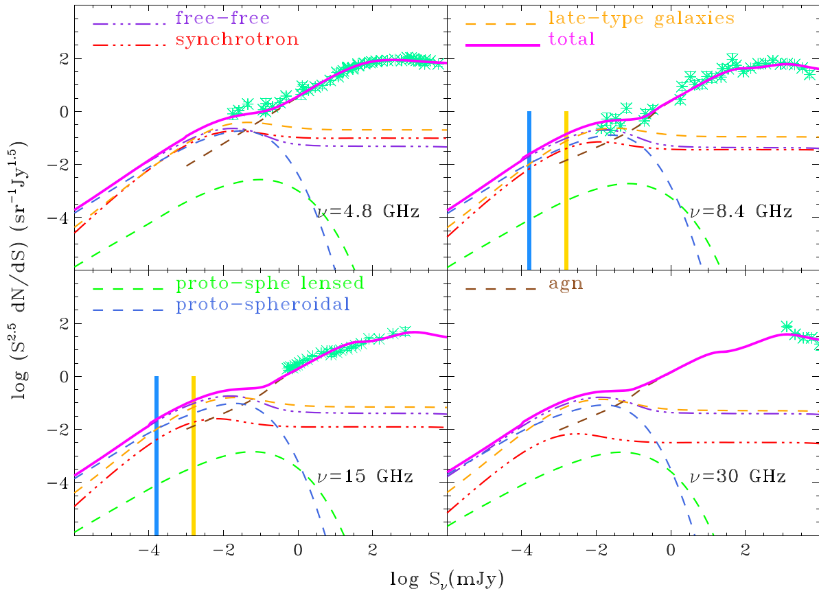
Figure 9. Predicted vs. observed counts at 4.8, 8.4, and 30 GHz. Dusty galaxies come up at sub-mJy flux density levels and their counts are accounted for by the model. At higher flux densities the counts are dominated by canonical, AGN-powered radio sources. The models shown are from Massardi et al. (2010) at 1.4, and 4.8 GHz and from de Zotti et al. (2005) at 8.4 and 30 GHz. The various lines correspond to the contributions from the different source populations (dashed yellow lines: late-type galaxies; dashed blue lines: unlensed proto-spheroidal galaxies; dashed green lines: strongly lensed proto-spheroidal galaxies; dashed brown lines: radio-loud AGNs; solid magenta line: total) and from the different emission processes (triple-dot dashed lines, red for synchrotron, violet for free-free). The solid vertical lines indicate the predicted flux density limits, for unresolved sources, of possible deep (yellow) and ultra-deep (blue) band 5 surveys with SKA1-MID.
