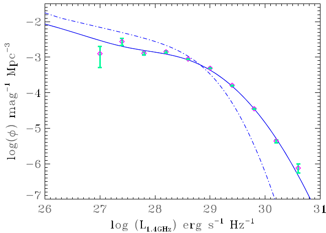
Figure 4. Synchrotron luminosity function of local star-forming galaxies derived from the local SFR function using the nonlinear L_{\text{radio}} –SFR relation (see Equation (4)) and a dispersion of \sigma_{\text{radio}} = 0.4 dex around the mean relation, compared with the observational determination by Mauch & Sadler (2007). The luminosity function obtained assuming a simple proportionality between L_{\text{radio}} and the SFR (Equation (3)) is also shown for comparison (dot-dashed line). The dispersion \sigma_{\text{radio}} raises the bright portion of the luminosity function while Equation (4) flattens the faint part.
