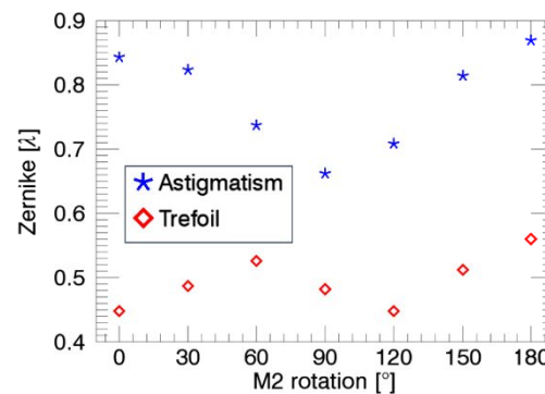
Figure 9. Dependence of astigmatism and trefoil on M2 rotation, with values corrected for temperature. As foreseen, astigmatism shows a minimum every 180^{\circ} , while trefoil every 120^{\circ} . To reduce the total PtV, the orientation of M2 minimizing astigmatism was selected.
