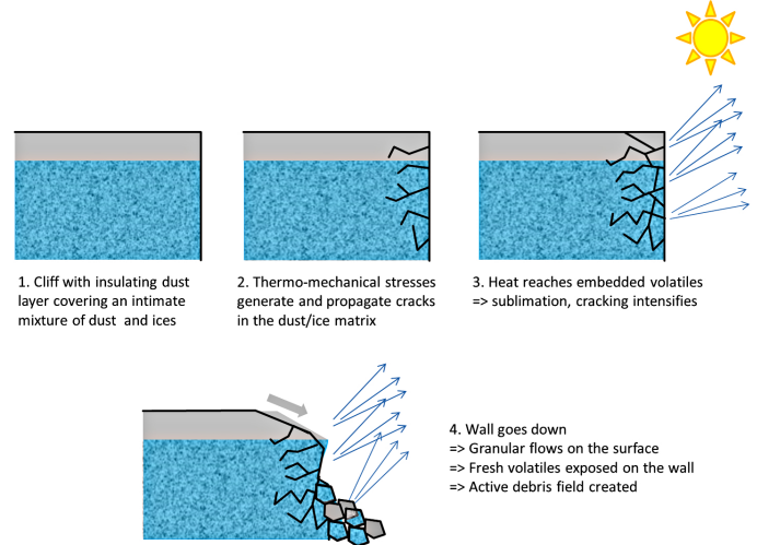
Fig. 4. Scenario of surface evolution describing how the regressive erosion of cliffs can expose volatiles and lead to localized activity.
