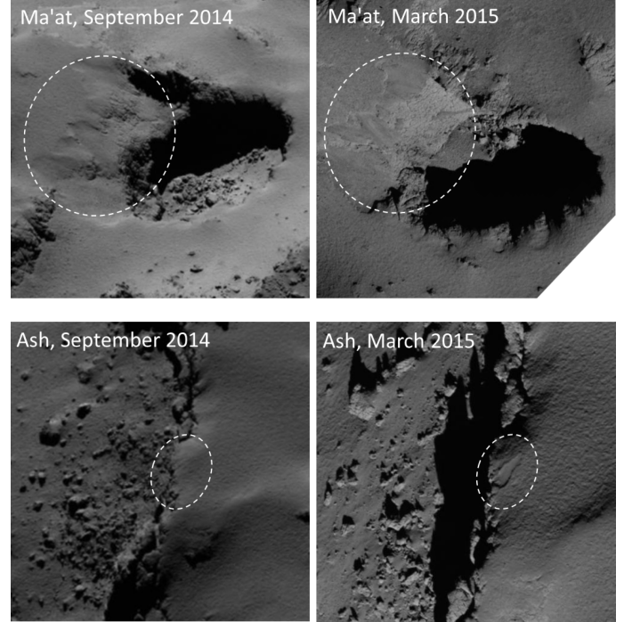
Fig. 8. Evolving flows observed in September 2014 and March 2015. Top panel: flows from Ma'at regions between two of the active pits have changed; their outline is different and they seem to have expanded laterally. Bottom panel: new flow in Ash region, following the partial collapse of one active cliff. Image references for top panels : NAC_2014-09-12T01.33.04.375Z_ID30_1397549400_F22 & NAC_2015-03-28T16.18.50.365Z_ID10_1397549000_F82; and bottom panels : NAC_2014-09-10T18.34.00.345Z_ID30_1397549000_F22 & NAC_2015-03-28T14.19.49.405Z_ID10_1397549000_F82).
