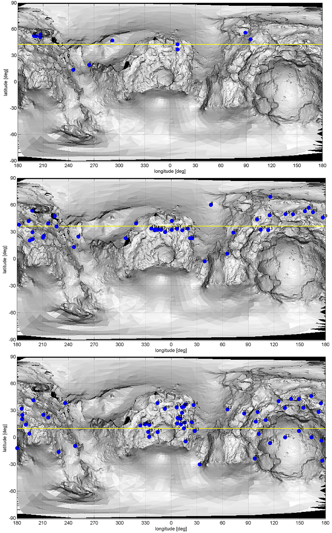
Fig. A.5. Maps of active sources obtained at three different epochs. From top to bottom: september 2014, November 2014, April 2015. The map is shaded according surface slopes, accounting for gravity and centrifugal force. White is flat, black is a vertical wall. The yellow line marks the subsolar latitude. These maps are not an exhaustive catalog of all sources, see Sect. 3
