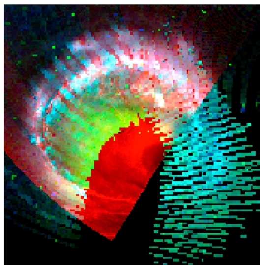
Figure 1. RGB spectrometer-imager composition of the southern aurora. The red channel comes from an imager acquisition of the aurora (4.54–5.02 \mu\text{m} ). Green is set at 3.31 \mu\text{m} where the \text{H}_3^+ emission is overlaid to the \text{CH}_4 Q branch, and blue is set at 3.54 \mu\text{m} , a \text{H}_3^+ emission band. The green and blue channels are composed from the spectrometer's data. The spectral data do not completely cover the imager acquisition. Colors would be affected by both brightness and relative amplitude of the RGB bands. Black corresponds to the absence of data.
