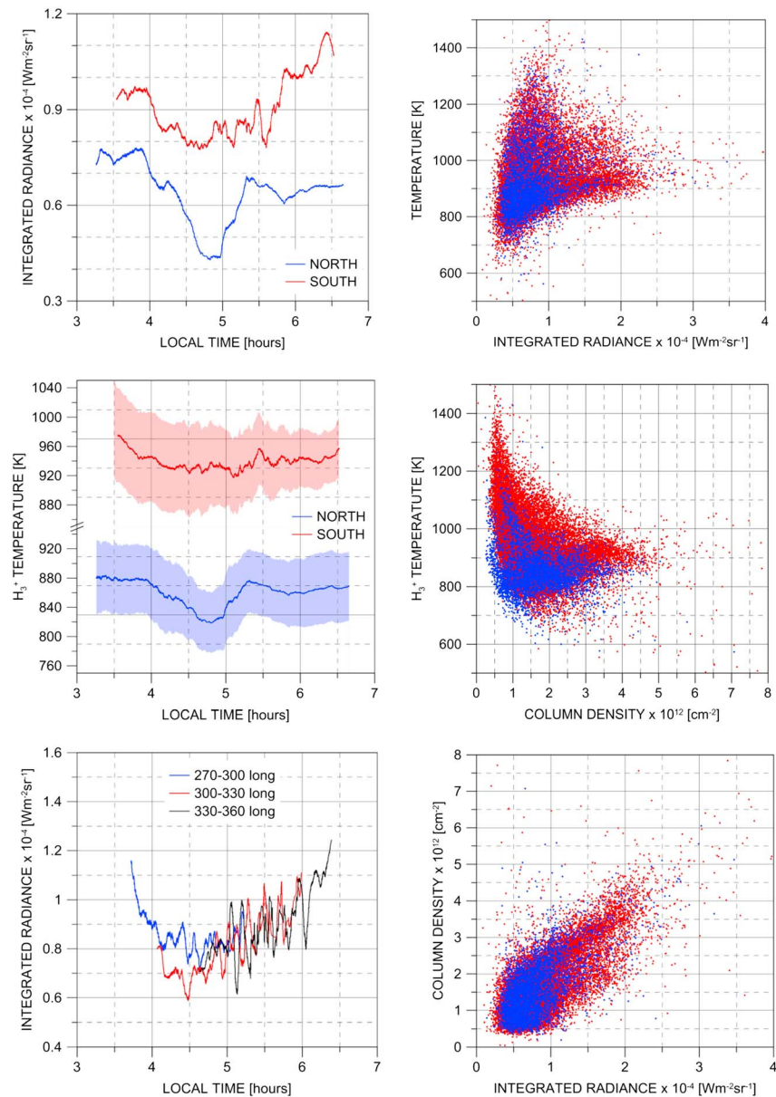
Figure 5. (left column, top) Local time dependence of the H 3 + integrated radiance (emissions in the range 3.35 and 3.75 \mu\text{m} ) versus the Jovian time of the day; (left column, middle) H 3 + effective temperature versus the Jovian time of the day, the colored regions account for the respective retrieval errors on the temperature; (left column, bottom) trends of the integrated radiances during the Jovian day in three different longitudinal sectors of the southern aurora. The error on the integrated radiances reported in the panels is less than 0.7 \times 10^{-5} \text{ W m}^{-2} \text{ sr}^{-1} . (right column, top) Scatterplots between temperature and integrated radiance, (right column, middle) temperature and column density, and (right column, bottom) column density and integrated radiance. In the scatterplots the northern auroral data are shown in blue and southern ones are in red.
