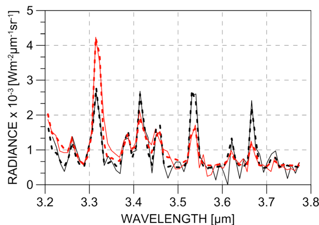
Figure 3. Spectra collected in the area of the auroral oval (black curve) and in the inner part of the oval (red curve). The dashed curves are the corresponding modeled spectra obtained by the retrieval method from Dinelli et al. [2017] and used for computing \text{H}_3^+ temperatures and column densities. The error on the observed values (not shown) is 1.5 \times 10^{-4} \text{ W m}^{-2} \mu\text{m}^{-1} \text{ sr}^{-1} .
