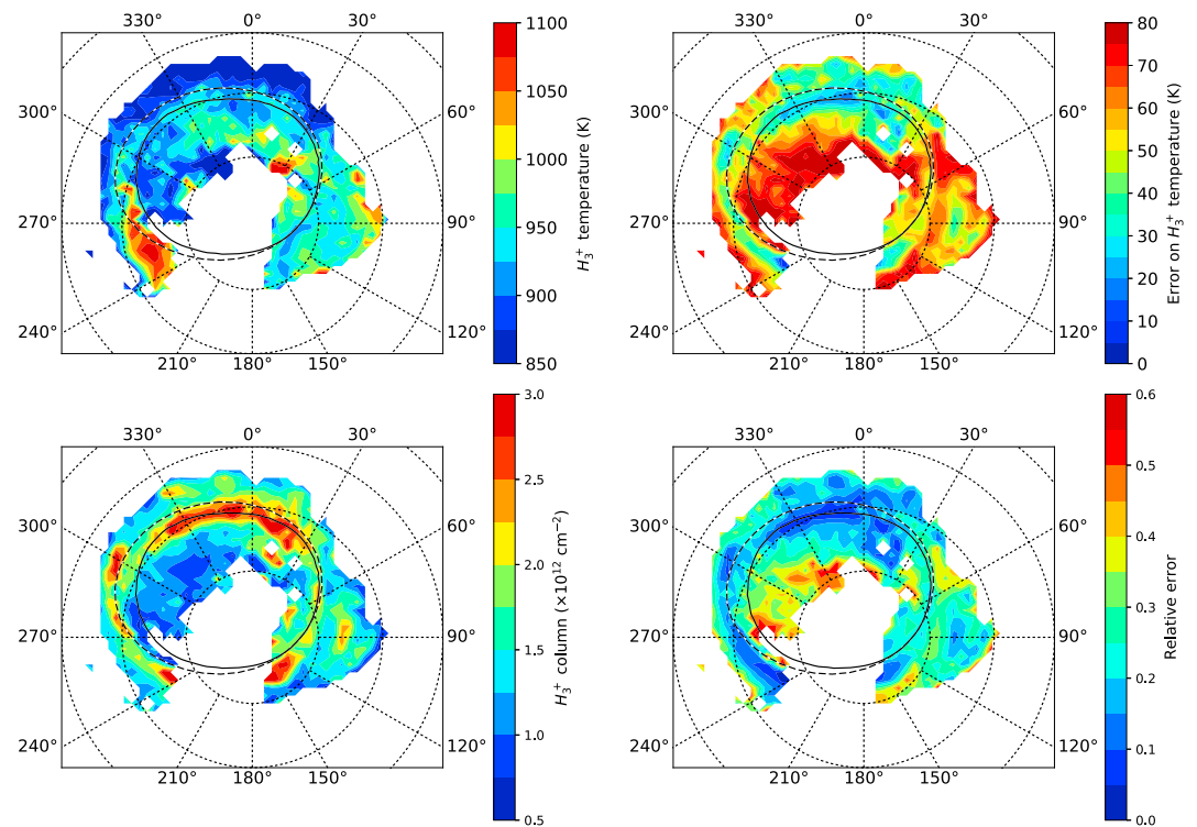
Figure 4. (top left) \text{H}_3^+ effective temperature and (top right) error on its retrieval. (bottom left) \text{H}_3^+ column density and (bottom right) error on its retrieval. The continuous oval curve is from VIP4 model [Connerney et al. , 1998]; the dashed curve is the UV statistical oval reported by Grodent et al. [2003]. Latitude lines are spaced by 10^\circ . The orthographic projection that contains the 60^\circ latitude south circle is divided into 50 \times 50 bins for each map. Then, all the measurement points falling in each single bin are averaged to produce the contour plots shown in the figure.
