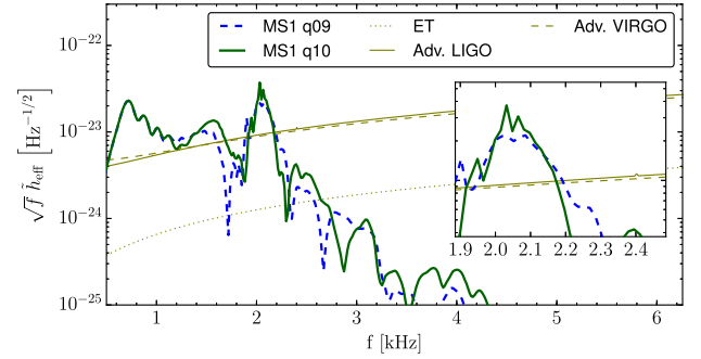
FIG. 28. Like Fig. 27, but for the MS1 models.
