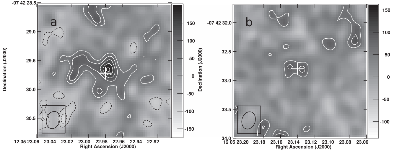
Figure 6. Moment zero images of BRI 1202–0725 made with the B-configuration data tapered to 750 k \lambda (B750), averaged over the width of the CO( J = 2 \rightarrow 1 ) line as seen in B750. Contours begin at \pm 2\sigma and are in steps of 1\sigma . 44 GHz continuum positions of this work are shown by crosses (size of \sim 0''.2 corresponds to positional uncertainty). The restoring beam ( 0''.31 \times 0''.23 ) at position angle -17^\circ is shown as an ellipse in the lower left corner. (a) Image of the SMG, 1\sigma = 32.3 \text{ mJy beam}^{-1} \text{ km s}^{-1} . (b) Image of the QSO, 1\sigma = 28.8 \text{ mJy beam}^{-1} \text{ km s}^{-1} . The grayscale is in units of \text{mJy beam}^{-1} \text{ km s}^{-1} .
