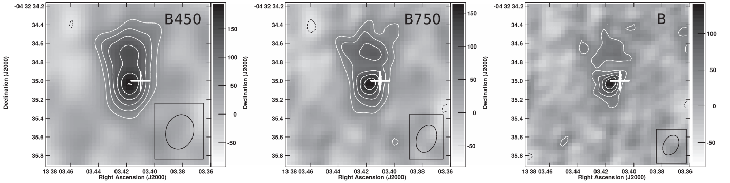
Figure 7. Moment zero images of BRI 1335–0417 made with tapered and untapered B-configuration data, integrated over the width of the CO( J = 2 \rightarrow 1 ) line. The location of continuum emission from this work is shown by crosses (size of \sim 0''.2 corresponds to positional uncertainty based on our beam size). Contours begin at \pm 2\sigma and are in steps of 1\sigma . The restoring beams are shown in the lower right corner. The grayscale is in units of \text{mJy beam}^{-1} \text{ km s}^{-1} . Left: B-configuration tapered to 450 k \lambda , 1\sigma = 27 \text{ mJy beam}^{-1} \text{ km s}^{-1} . The restoring beam is ( 0''.38 \times 0''.29 ) at position angle -15^\circ . Middle: B-configuration tapered to 750 k \lambda , 1\sigma = 24 \text{ mJy beam}^{-1} \text{ km s}^{-1} . The restoring beam is ( 0''.30 \times 0''.21 ) at position angle -20^\circ . Right: untapered B-configuration, 1\sigma = 23 \text{ mJy beam}^{-1} \text{ km s}^{-1} . The restoring beam is ( 0''.23 \times 0''.15 ) at position angle -27^\circ .
