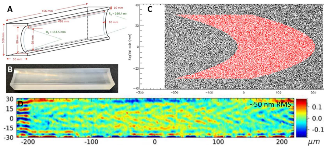
Figure 4. A. Drawing of the workpiece. B. Mirror blank manufactured at Carl Zeiss SMT GmbH. C. Projection area (red area) of the BEaTriX beam expander back traced to the paraboloidal mirror surface area. D. Longitudinal error map after bonnet polishing [13].
