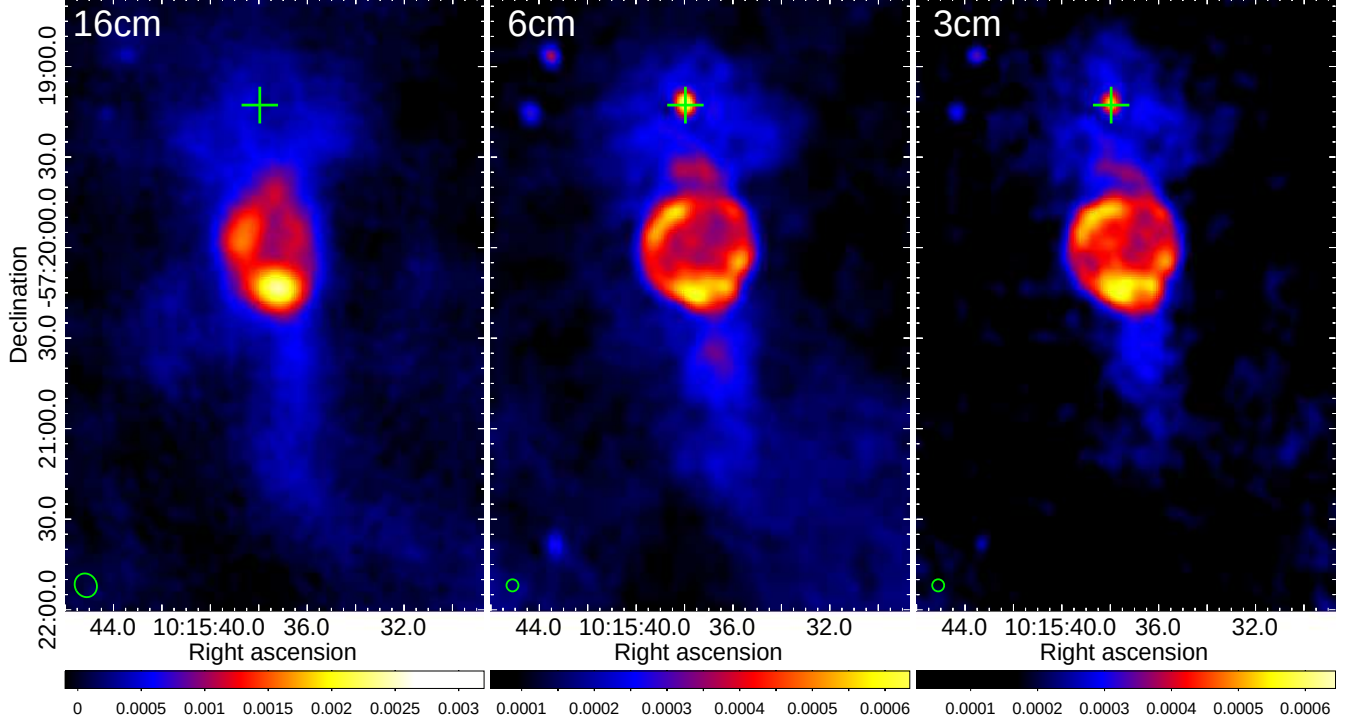
FIG. 2.— ATCA radio intensity maps zoomed in at J1015 and the nebula G283.1–0.59 at 16, 6, and 3 cm. The 16 cm image is obtained from the off-pulse phase bins with the pulsar binning data (see Figure 4 for the pulse profile of J1015.) The crosses mark the pulsar position and the beam sizes are shown in the lower left. The color bars are in units of \text{Jy beam}^{-1} .
