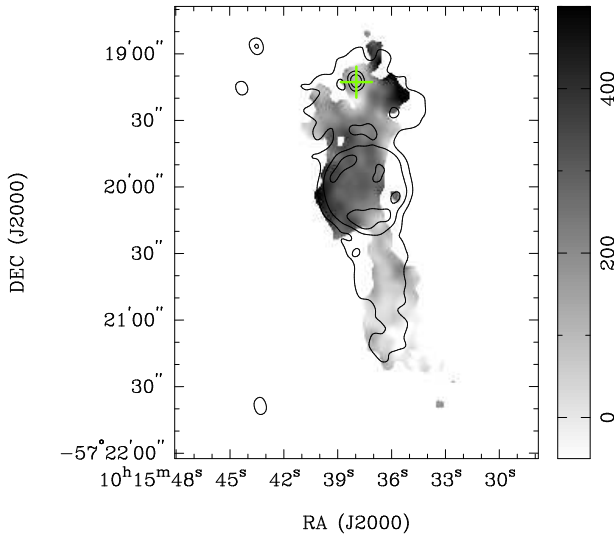
FIG. 7.— RM distribution in G283.1–0.59 obtained by comparing the 6 and 3 cm polarization angles. The contours are from the 6 cm total intensity map at levels of 0.2, 0.35, and 0.5 mJy beam −1 . The typical uncertainty is about 50 rad m −2 and the map is clipped where the uncertainty > 80 rad m −2 . The gray scale is linear, ranging from −50 to 500 rad m −2 . The cross marks the pulsar position.
