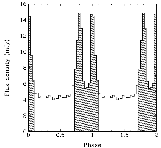
FIG. 4.— Pulse profile of J1015 obtained with the 16 cm pulsar binning observation. Two cycles are plotted and the shaded and unshaded regions denote the on- and off-pulse phases, respectively, chosen for the pulsed flux density measurement. An image formed with the off-pulse phase is shown in Figure 2.
