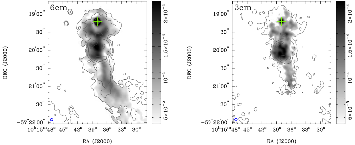
FIG. 6.— Linearly polarized intensity of G283.1–0.59 at 3 and 6 cm, overlaid with total intensity contours at levels of 0.15, 0.2, 0.35, and 0.5 mJy beam −1 . The maps are clipped where the polarized intensity has S/N < 3 or the total intensity has S/N < 10. The gray scales are linear, ranging from 0.03 to 0.22 mJy beam −1 . The crosses mark the pulsar position and the beam sizes are shown in the lower left.
