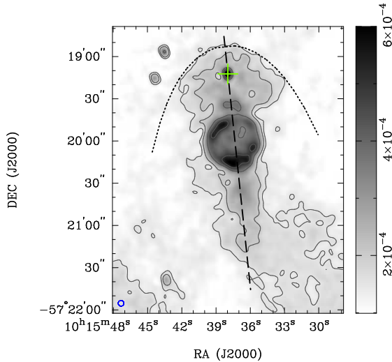
FIG. 3.— The same 6 cm intensity map of J1015 and G283.1–0.59 as in Figure 2, overlaid with intensity contours at levels of 0.15, 0.2, 0.35, and 0.5 \text{ mJy beam}^{-1} . The dotted curve shows a theoretical model of a classical bow shock (Wilkin 1996) and the dashed line indicates its axis of symmetry. The cross marks the pulsar position and the beam size is shown in the lower left. The gray scale is linear and the color bar is in units of \text{Jy beam}^{-1} .
