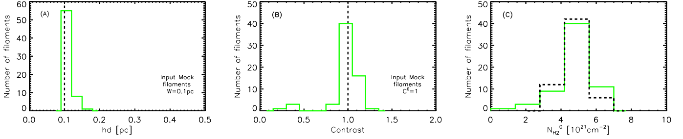
Fig. B.1. Histograms of derived crest-averaged properties (half-power diameter, hd , in panel a ; filament contrast, C^0 , in panel b ; background-subtracted central column density, N_{H_2}^0 , in panel c ) in measurement tests using a population of Gaussian mock filaments. The vertical dashed lines in panels a and b indicate the fixed input properties of the mock filaments: FWHM width ( W=0.1 pc) and column density contrast ( C^0=1 ). In panel c , the black and green histograms show the distribution of input and derived background-subtracted column densities averaged along the filament crests, respectively.
