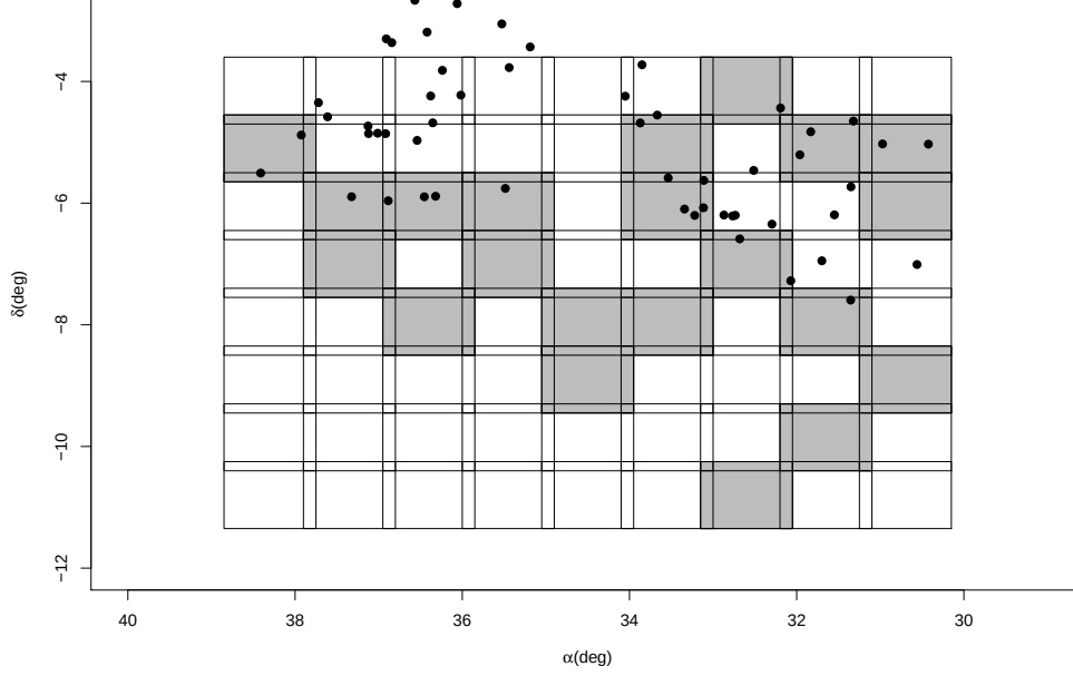
Fig. 1. Overlap of XXL-100-GC with the CFHTLenS W1 field. The boxes are individual pointings in CFHTLenS with XXL-North field clusters (filled points). The shaded boxes are pointings that fail the CFHTLenS weak-lensing field selection criteria (See section 4.1).
