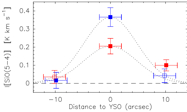
Fig. 4. Integrated intensities of the SiO(5–4) EHV emission (both blue and red components) measured at three positions along the L1157 outflow axis. The negative and positive distances correspond to the blue and red outflow lobes. The dotted curves are Gaussians with the size of the telescope beam at the SiO(5–4) frequency. A nominal rms position uncertainty of 2'' has been assumed for all positions.
