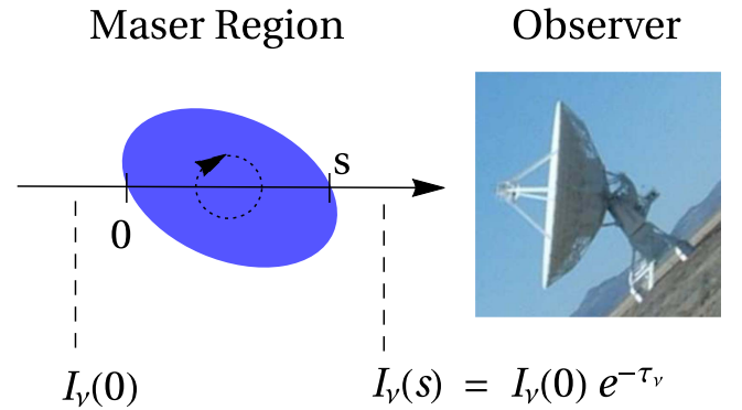
Figure 9. Simple model used to explain the observed variability. As the maser region slowly rotates, a different amplification path ( 0 \rightarrow s ) results in a change in the maser gain ( \tau_v ), and thus, a change in the observed intensity.
