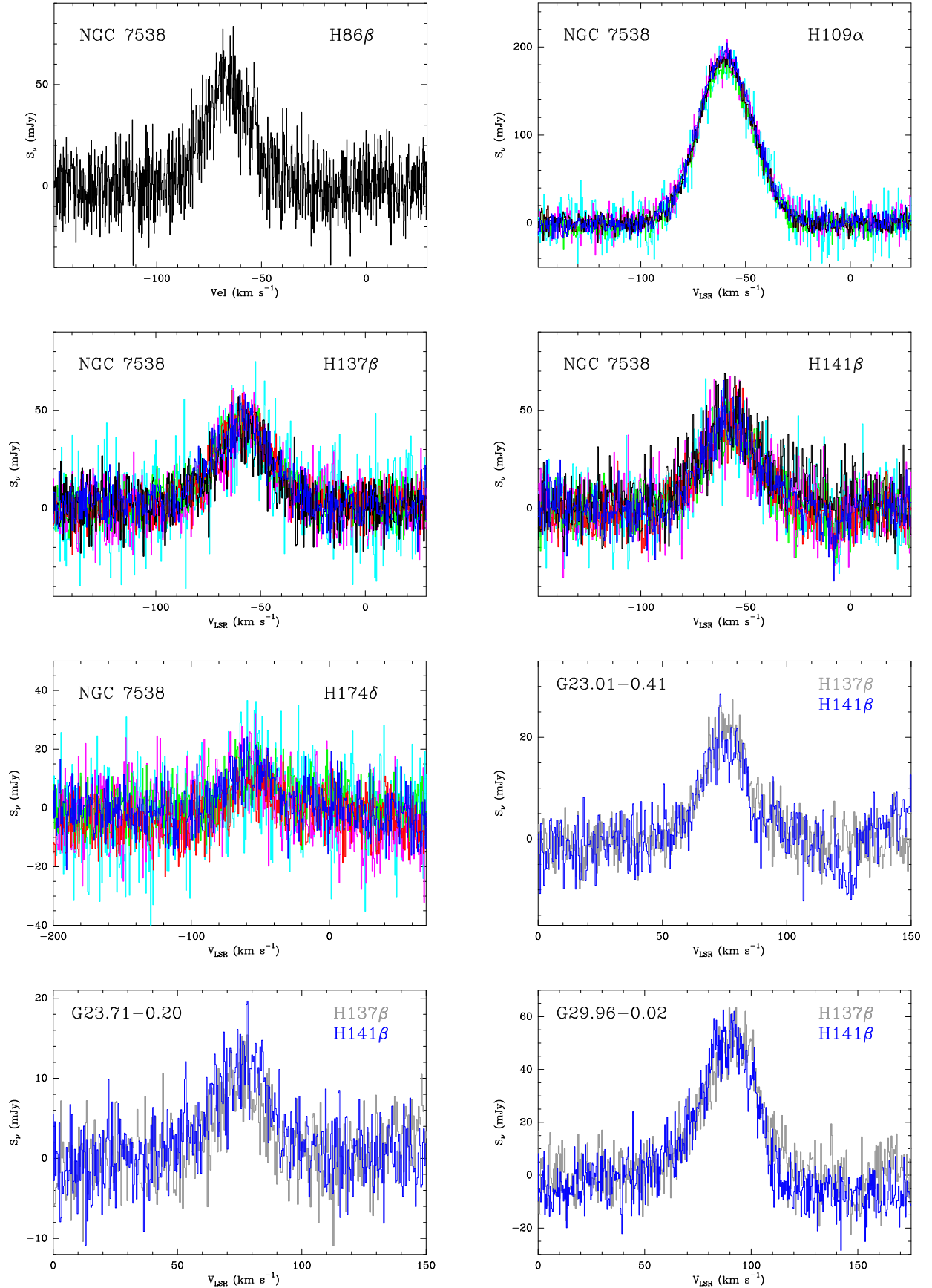
Figure 7. Radio recombination lines detected in this project. The NGC 7538 panels show specific radio recombination line transitions, and different colors represent different observing epochs: 2008 May (epoch 1; black), 2009 May (epoch 2; red), 2009 July (epoch 3; green), 2009 July (epoch 4; blue), 2010 May (epoch 5; pink), and 2011 May (epoch 6; magenta). Not all lines were observed in all epochs (see Table 1). The panels of G23.01-0.41, G23.71-0.20, and G29.96-0.02 show two different recombination line transitions (H137β in gray; H141β in blue) that were observed in epoch 4 (2009 July 17).
