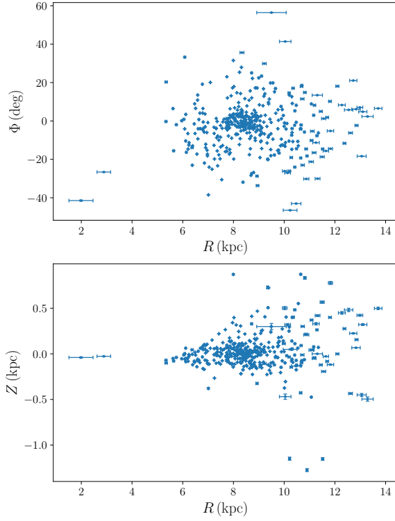
Fig. 10. Spatial distribution of the high-quality sample in Galactic cylindrical coordinates.
