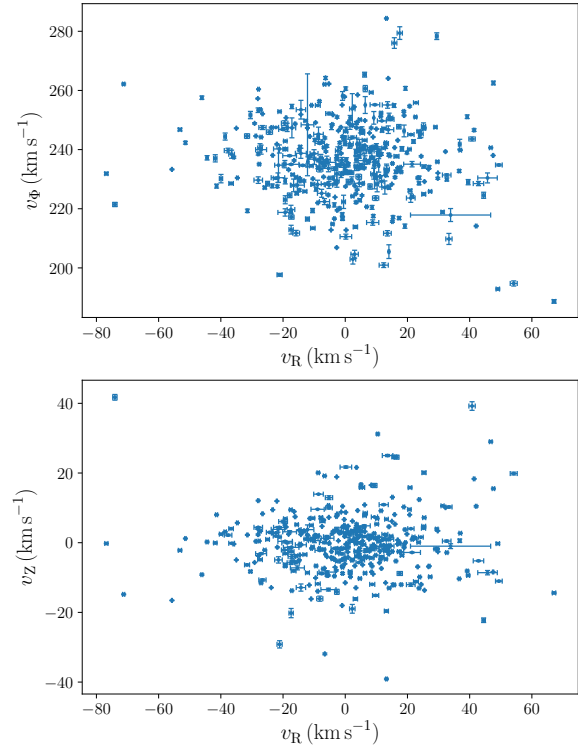
Fig. 11. Velocity distribution of the high-quality sample in Galactic cylindrical coordinates. BH 222 and BH 140 are not represented (see text).
