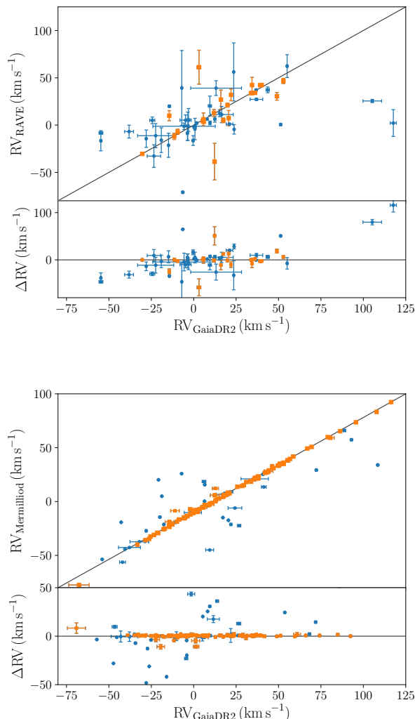
Fig. 5. Comparison of mean RV from Gaia DR2 with those from Conrad et al. (2014) using RAVE data (upper panel) and from Merriliod et al. (2008, 2009) (lower panel). The OCs with at least three members in each catalogue are shown in orange. The error bars combine the uncertainties of both catalogues.
