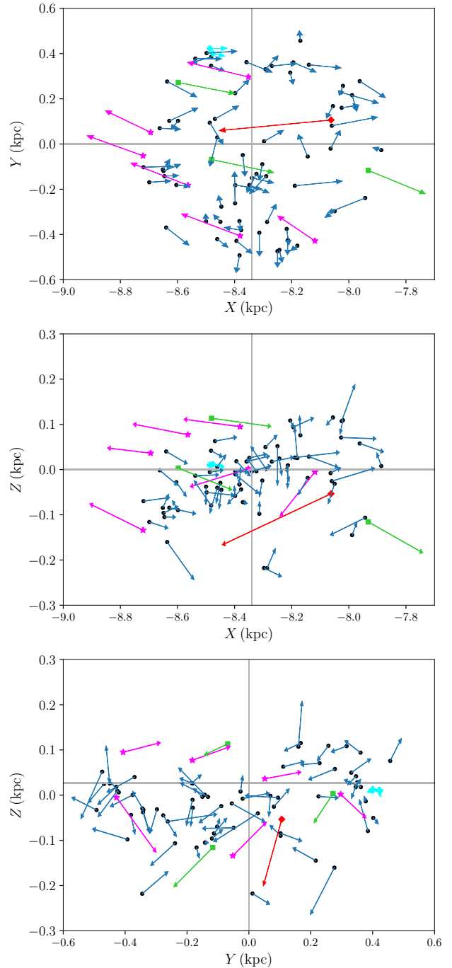
Fig. 7. Galactic position in (X, Y) (upper panel) and (X, Z) (middle panel) and (Y, Z) (bottom panel) for the high-quality OC sample closer than 500 \text{ pc} . The size and angle of the arrows are proportional to (V_R, V_\phi - V_c) , (V_R, V_Z) , and (V_\phi - V_c, V_Z) . The horizontal and vertical lines indicate the position of the Sun. Several objects discussed in the text are represented by different symbols and colours. The red diamond represents Ruprecht 147, the green squares show Mamajek 4, NGC 2632, and Stock 2 (Group 1 in Table 2), the magenta stars show Turner 5, NGC 7092, ASCC 41, NGC 1662, Ruprecht 98, and Stock 10 (Group 2 in Table 2), and the blue circles indicate RSG 7 and RSG 8.
