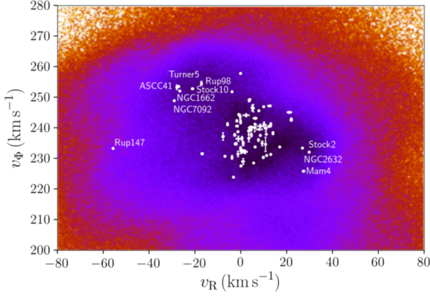
Fig. 8. Velocity distribution of nearby OCs (dist \leq 500 pc) in (V_R, V_\phi) , superimposed on field stars in the same volume around the Sun taken from Gaia Collaboration et al. (2018c). The most extreme OCs are indicated, in particular, the two groups listed in Table 2.
