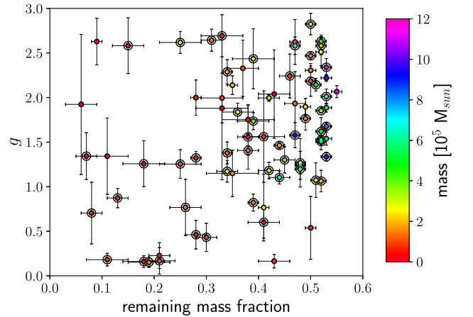
Figure 16. Comparison between the remaining mass fraction \mu from Balbinot & Gieles (2018) and the LIMEPY truncation parameter g . Lower values of \mu indicate a larger fraction of the cluster has been lost, consistent with a more evolved cluster. Colours indicate the cluster mass from Harris (1996, 2010 version). GCs with large ( >0.1 per cent) fractions of PEs are shown as points with an additional circle around them.
