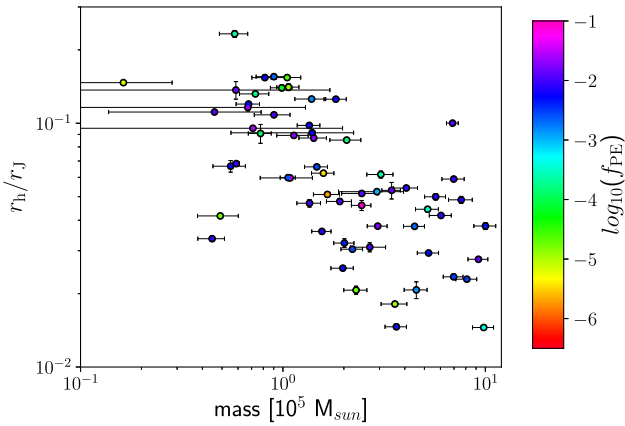
Figure 17. Comparison between the mass of the clusters from Harris (1996, 2010 version) and the ratio r_h/r_j from the LIMEPY models. The colour of individual points indicates the value of f_{PE} from SPES models.
