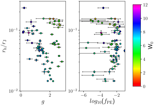
Figure 15. Comparison between the ratio r_h/r_J and g or f_{PE} for the LIMEPY and SPES models, respectively. The colour of individual points indicates the value of W_0 .
