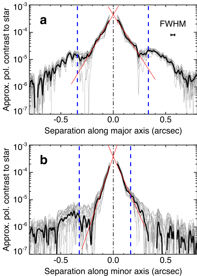
Figure 3. Polarized surface brightness profiles for the LkCa 15 disk. (a) Profile of the Q_\phi image along the major axis averaged over a width of 21 pixels ( \approx 76 mas) centered on the star (thick black curve). The family of thin gray curves are obtained by adding similar profiles taken in the U_\phi image at various position angles to the black curve, and therefore visualize the noise level in the data. The contrast of a given pixel is calculated by the ratio of its value and the maximum pixel in the stellar full-intensity PSF. The normalization is approximate due to the stellar PSF being saturated in some exposures. The blue dashed lines mark the location of the light blue fit ellipse in Figure 2. The red lines are exponential fits to the inner scattering component. Positive separation values correspond to the western side of the disk. The size of the PSF’s FWHM is given for comparison. (b) Profile of the Q_\phi image along the minor axis averaged over a width of 81 pixels ( \approx 292 mas) centered on the star. Positive separation values correspond to the northern side of the disk.
