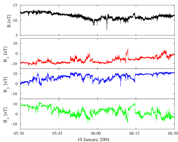
Figure 1. Solar wind magnetic field measurements during the time interval 05:30–06:30 UT on 10 January 2004. Data are obtained from Cluster 3 at the time resolution of 8.9 ms.
