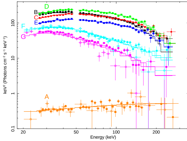
FIG. 4.— Spectra measured for different phases: a low state spectrum (A) and spectra measured during the most intense flare (B to G). Circles denote data from SPI; squares from IBIS/ISGRI.
