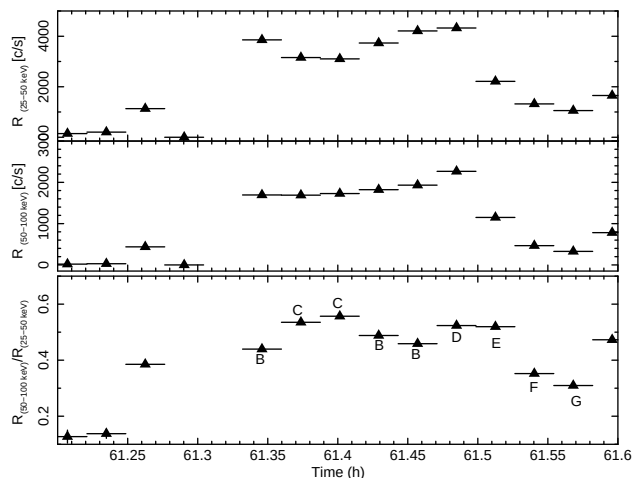
FIG. 2.— Light curves of the major flare in the 25-50 keV (top panel) and 50-100 keV (center panel) bands. Start time is MJD 57190, 21:30:45:186 UT. The hardness ratio in the two bands is shown in the bottom panel. Periods B to G mark the intervals used for the spectral analysis (see text for details).
