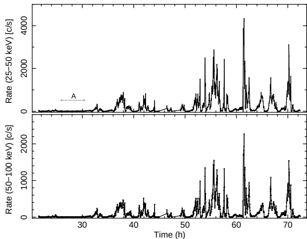
FIG. 1.— Light curve with IBIS/ISGRI count rates in the 25-50 keV and 50-100 keV energy bands, for the data period spanning revolution 1554. Start time is MJD 57190, UTC 21:30:45:186.
