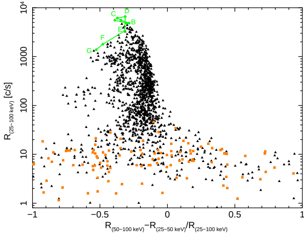
FIG. 3.— Intensity vs. hardness diagram for the full data set. Each point is generated using intensity values averaged over 100s. Square orange points at the bottom are integrated on period A, whereas green circle points (B to G) are taken during the most intense flare.
