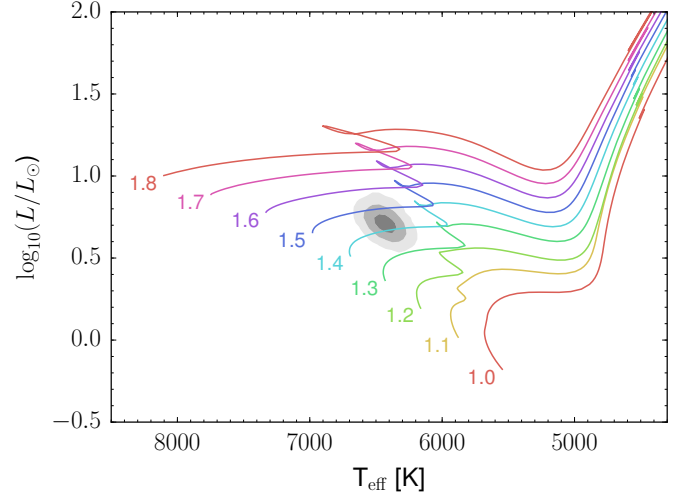
Fig. 9. Stellar evolution tracks from Dartmouth models, from the zero age main sequence stage to 25 Gyr age, in the luminosity-effective temperature plane for [\text{Fe}/\text{H}] = 0.15 . The results from the photodynamical modelling using stellar models are denoted by the grey contours corresponding to 39.3%, 86.5%, and 98.9% joint confidence regions. The mass in solar masses is annotated at the beginning of the main sequence of each track.
