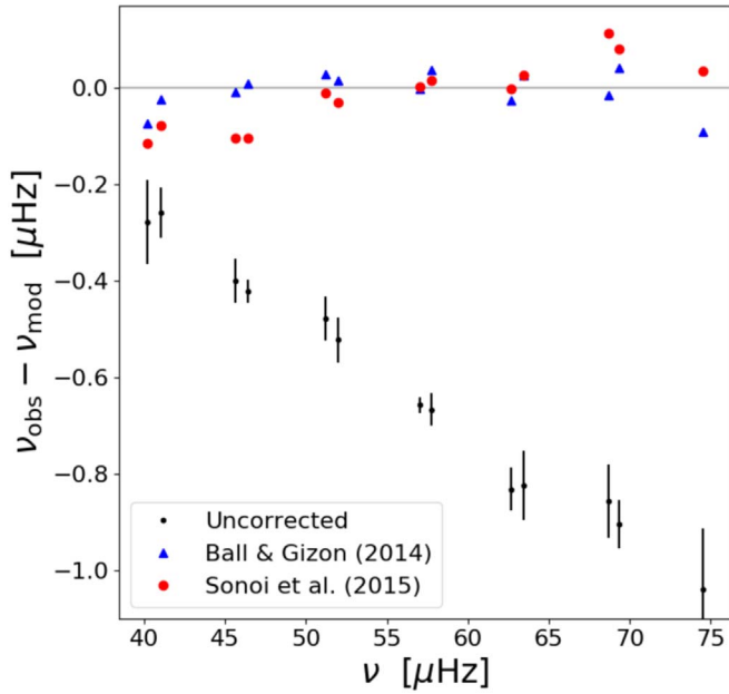
Figure 3. Difference between the observed frequencies and model frequencies (black), Ball & Gizon (2014) corrected frequencies (blue triangles), and Sonoi et al. (2015) corrected frequencies (red circles). The errorbars are shown for the uncorrected values only. Note the frequency-dependent trend left in the Sonoi et al. (2015) corrections.
