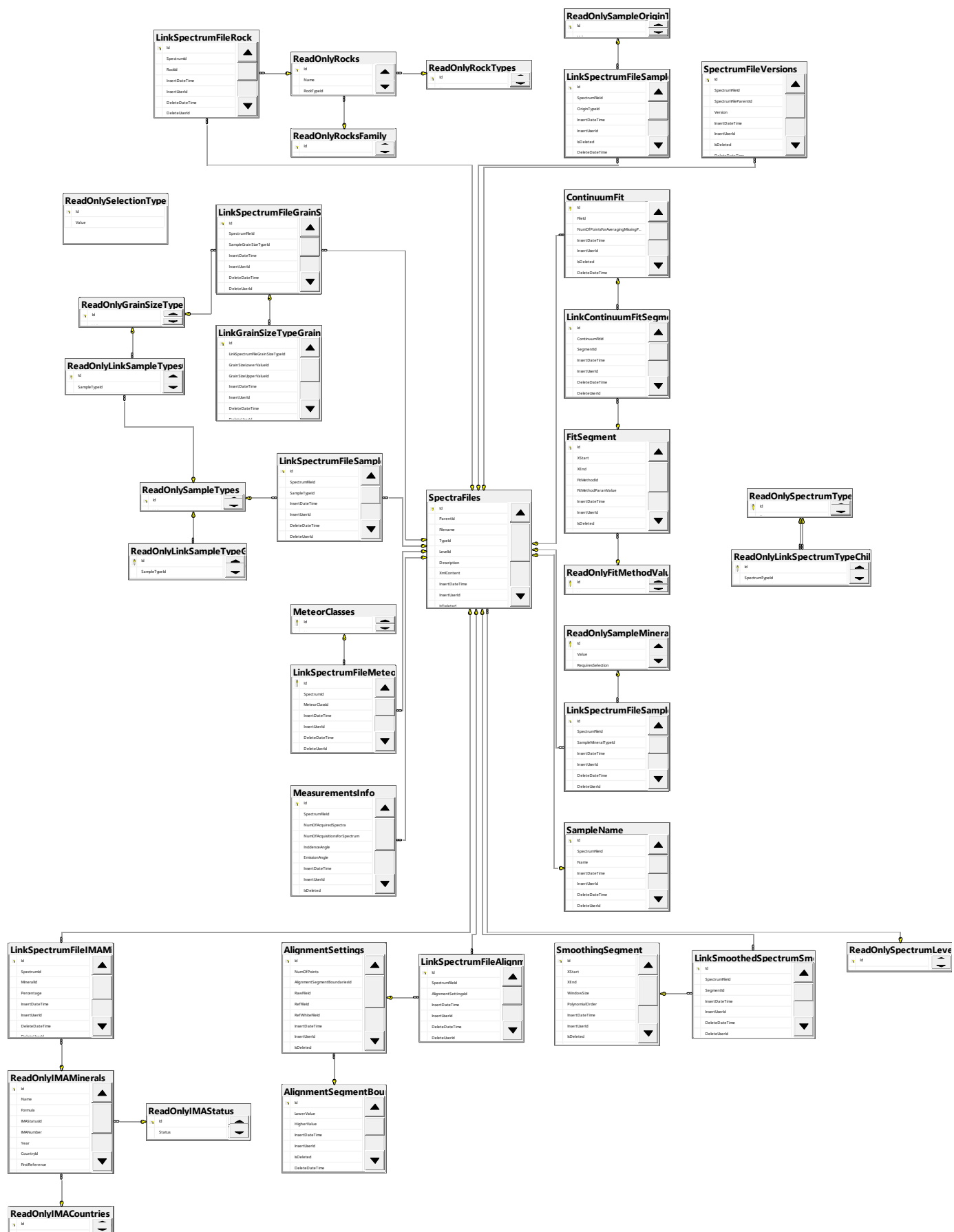
Figure 1 Schema of the SlabData database
