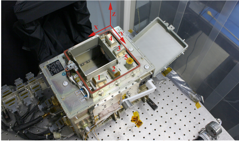
Figure 1: (a) Payload accommodated on the Rosetta spacecraft; GIADA is mounted on the nadir panel; (b) GIADA aperture where dust particles entering meet the GDS laser curtain and then impact on the IS at the bottom of the instrument; the five QCMs pointing in five different directions and forming the MBS are numbered in red.
