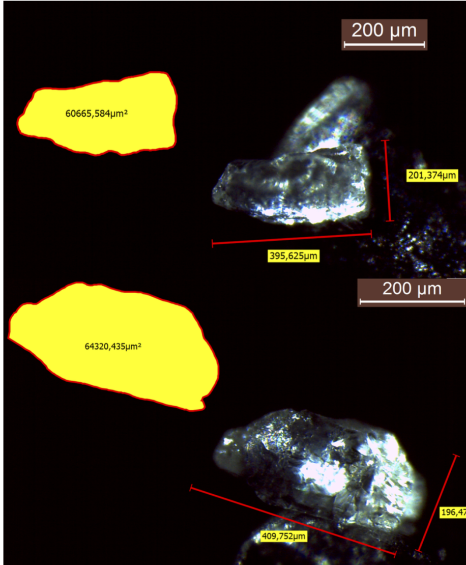
Figure 5: Two images of a forsterite grain belonging to the range 250-500 \mu\text{m} taken with the Leica IC80HD camera attached to the Leica MC205 Microscope. The measured geometrical cross section and the axes measured in the two positions are reported. The needle used to manipulate the particles is visible on the background of the samples.
