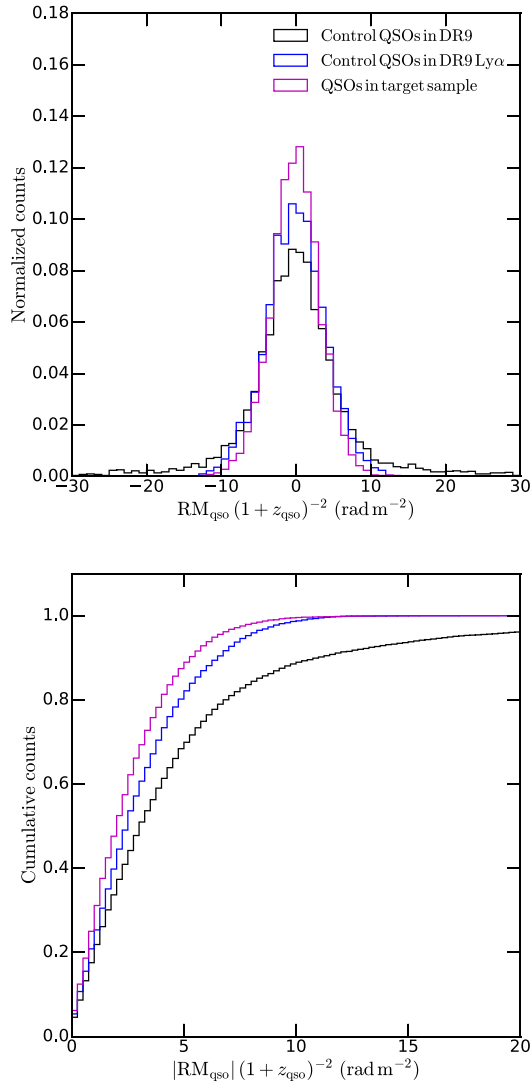
Figure 3. Top: Distribution of \text{RM}_{\text{qso}} (1 + z_{\text{qso}})^{-2} for different redshift coverages given in Fig. 2. Bottom: Cumulative distribution of |\text{RM}_{\text{qso}}| (1 + z_{\text{qso}})^{-2} . We assume that the intrinsic (rest-frame) RMs of the quasars follow a Gaussian distribution with zero mean and a standard deviation of 50 \text{ rad m}^{-2} . The distribution in black is for control quasars chosen from the entire SDSS DR9 catalogue, blue is for control quasars chosen from BOSS Lyman- \alpha forest catalogue, and magenta is for quasars in the target DLA sample.
