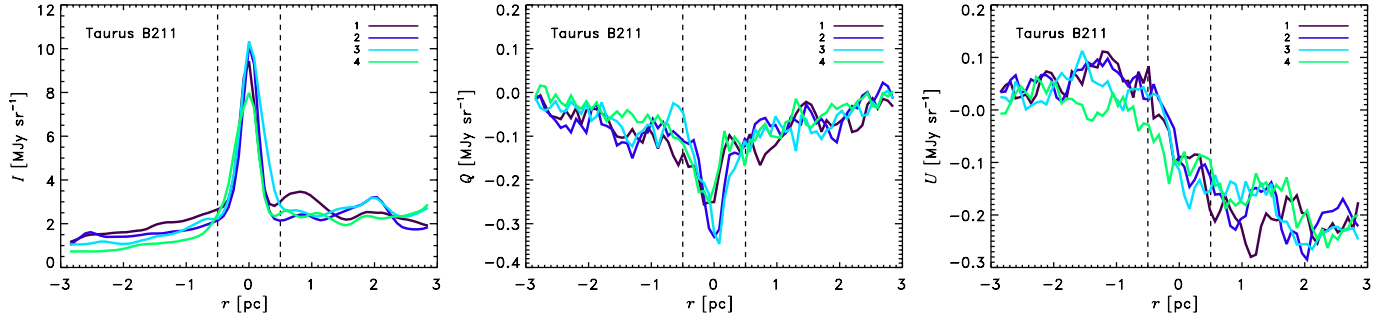
Fig. 5. Same as Fig. 2 for the Taurus B211 filament. Here r < 0 corresponds to the southern side of the filament axis. The filament is clearly seen in Q and is located in the area of a steep variation of the U emission. The dispersion of the emission is small along the length of the filament.
