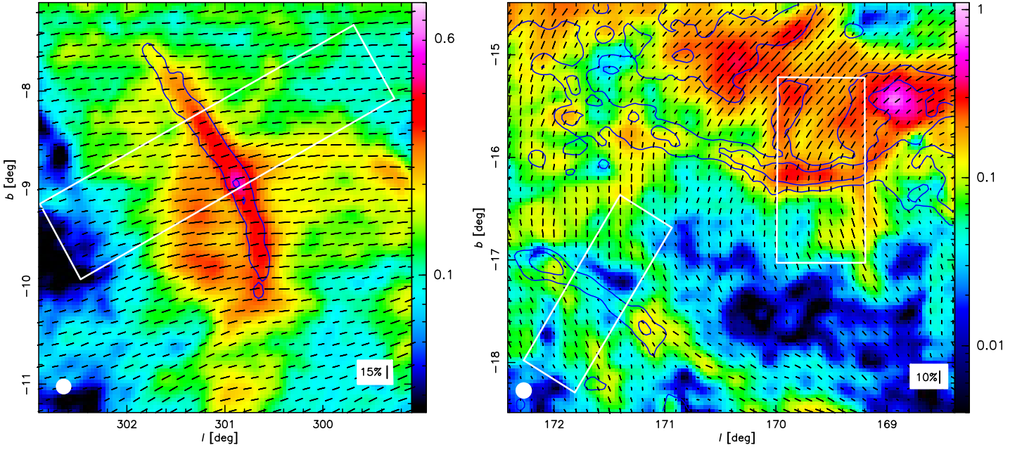
Fig. 7. Observed polarized emission at 353 GHz (in \text{MJy sr}^{-1} ) of the Musca (left) and Taurus (right) clouds. The maps are at the resolution of 9''.6 (indicated by the white filled circles) for increased S/N. The black segments show the \mathbf{B}_{\text{POS}} -field orientation ( \psi+90^\circ ). The length of the pseudo-vectors is proportional to the polarization fraction. The blue contours show the total dust intensity at levels of 3 and 6 \text{MJy sr}^{-1} , at the resolution of 4''.8 . The white boxes correspond to the area of the filaments and their backgrounds that is analysed in the rest of the paper.
