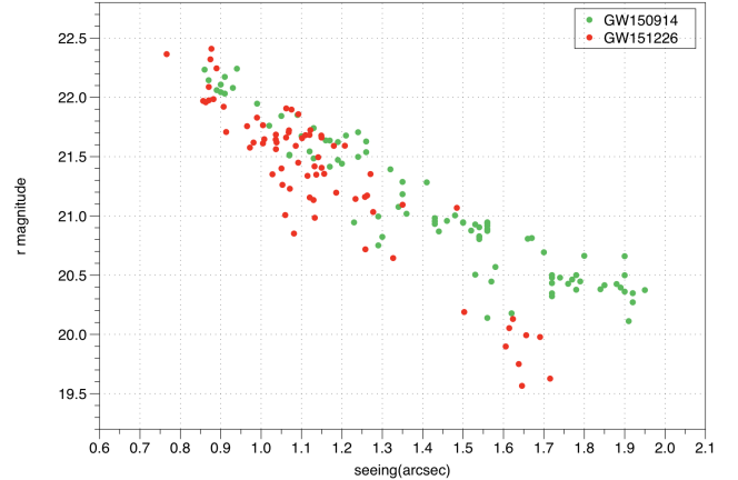
Figure 4. The limiting magnitude for transient detection ( DE_{50} ) as a function of seeing for the pointings of the two triggers discussed in this paper. The scatter is due to the fact that other factors are affecting the DE, first of all sky transparency.
