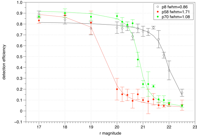
Figure 3. Example of the output of artificial star experiments. The detection efficiency (DE) is defined as the ratio between the number of detected stars and the number of injected stars in specific magnitude. The plot shows the correlation between DE and the magnitude for three pointings of GW151226 (p8, p58, p70).
