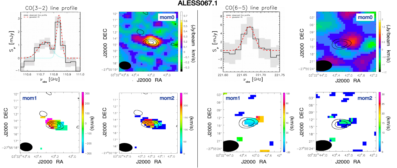
Figure 3. ALESS067.1 CO lines, i.e. J = 3 and J = 6 , in the order. The panels show: the observed spectral line profile (black solid line), the corresponding uncertainties on flux density (gray shaded area) and the (total) best Gaussian fit (dashed red line; in case of double peaked profile the two components are in cyan); the maps of the spectral line distribution momenta (mom0, mom1 and mom2) overlapped by the continuum contours at [2, 3, 4, 5] \times \sigma detected at the same frequency (ALMA B3 and ALMA B6, respectively). Black filled ellipse in the bottom left corners indicates the beam size.
