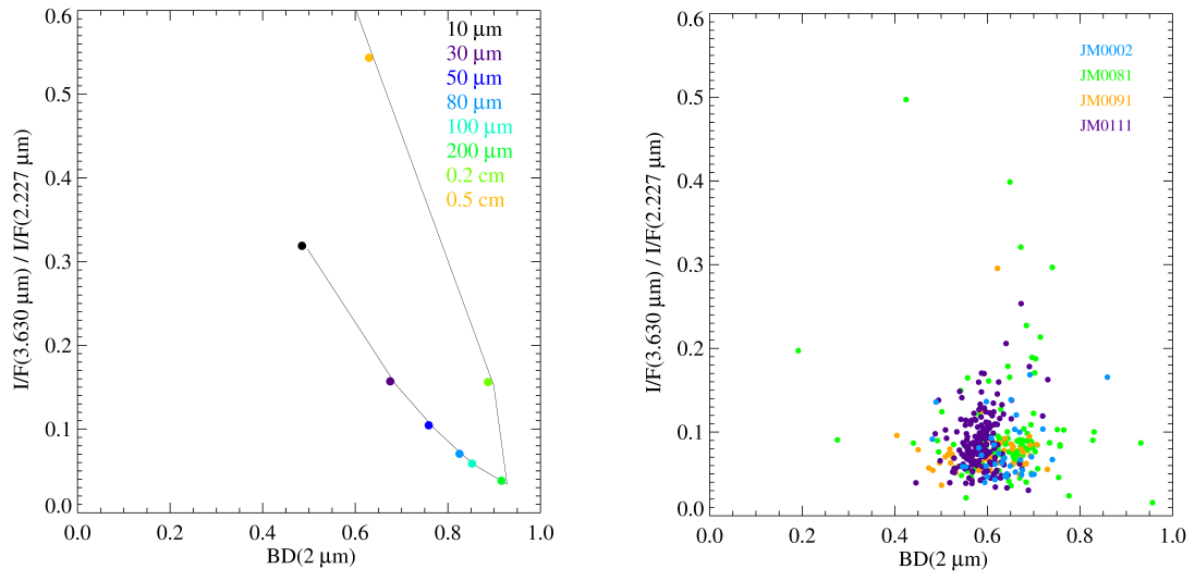
Figure 8: Left panel: trend of the BD(2 μm) and I/F(3.630 \mu\text{m}) / I/F(2.227 \mu\text{m}) as a function of water ice grain size. Right panel: distribution of JIRAM observations.
