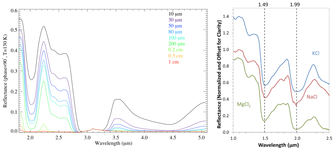
Figure 5: Left: synthetic spectra of water ice grains with sizes between 10\text{ }\mu\text{m} to 1\text{ cm} . Right: laboratory reflectance spectra of frozen eutectic chlorine salts \text{MgCl}_2 , \text{NaCl} , \text{KCl} at T=-30^\circ\text{C} (from Hanley et al. (2014) ).
