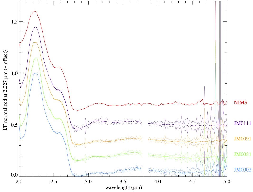
Figure 4: Europa's median I/F spectra collected during orbits JM0002, JM0081, JM0091, JM0111 compared with NIMS.
