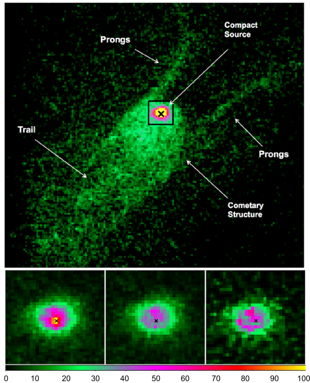
Figure 2. Top panel shows the unsmoothed Chandra ACIS image of the PWN region ( 2\frac{1}{6} across), corresponding to region 11 in Figure 1 (right). The black box is 20'' in size and indicates the zoomed-in region of the compact source shown in the bottom panel. The bottom panel's left image shows the unbinned image of the compact source, the middle panel shows the residual image after the subtraction of a point source at the location of the black "x," and the right panel shows the same residual deconvolved by the task arestore . The scale bar is the units of counts.
