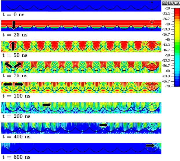
Figure 14. Snapshots of the electric field propagating through the array, when the antennas are excited by a plane wave coming from the zenith, at t = 0, 25, 50, 75, 100, 200, 400 , and 600 ns. The intensity of the E-field is expressed in \text{dBV m}^{-1} . Note how a part of the incident electromagnetic wave is reflected upwards and the other part towards the edge of the dishes. Then, the E-field propagates from one dish to the next one up to the end of the array, and with little attenuation.
