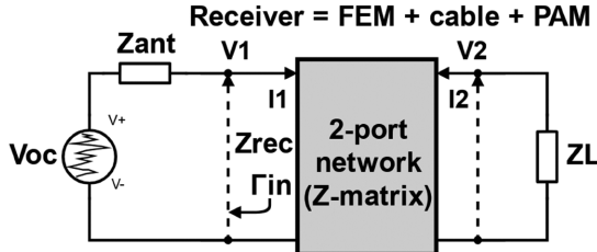
Figure 3. Equivalent electrical circuit of the antenna–RF receiver system.
