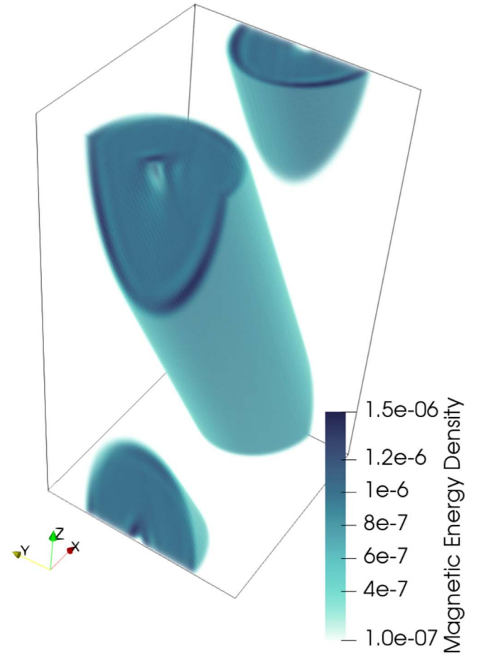
Figure 30. Magnetic field energy density B^2 of the magnetic field loop advection test in three dimensions with 128^2 \times 256 zones at time t = 2 . A threshold was imposed at 10^{-7} .
