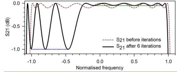
Fig. 6. Starting and final ripple of a 9 th order filter with uneven ripple.
