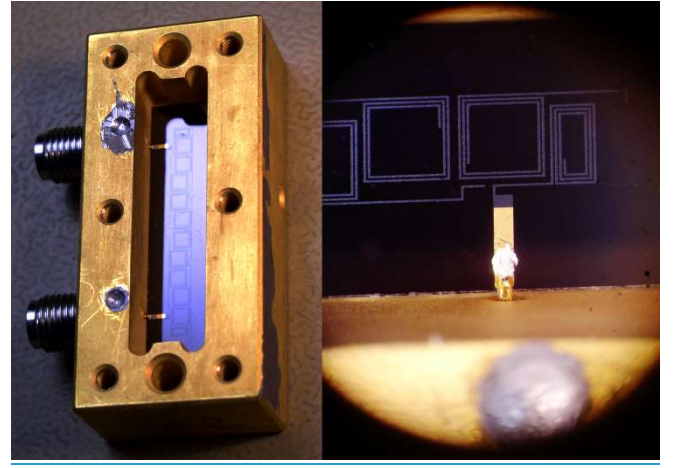
Fig. 9(a) The filter, fully assembled except for the cover, and (b) a close-up of the right-hand side. Contrast has been artificially enhanced to show the black spirals above the black ground plane. Nevertheless, in (a), it is the shadows of the spirals that are visible, rather than the spirals themselves.
