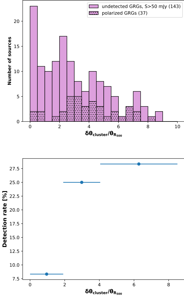
Fig. 7. Distribution of minimum distance from the closest foreground cluster for detected and undetected sources in polarization ( top panel ), and detection rate as a function of the minimum distance from foreground clusters ( bottom panel ). The widths of the bins were computed to contain the same total number of sources (i.e., 60). Markers were positioned at the center of each bin and the error bars show the width of the bins.
