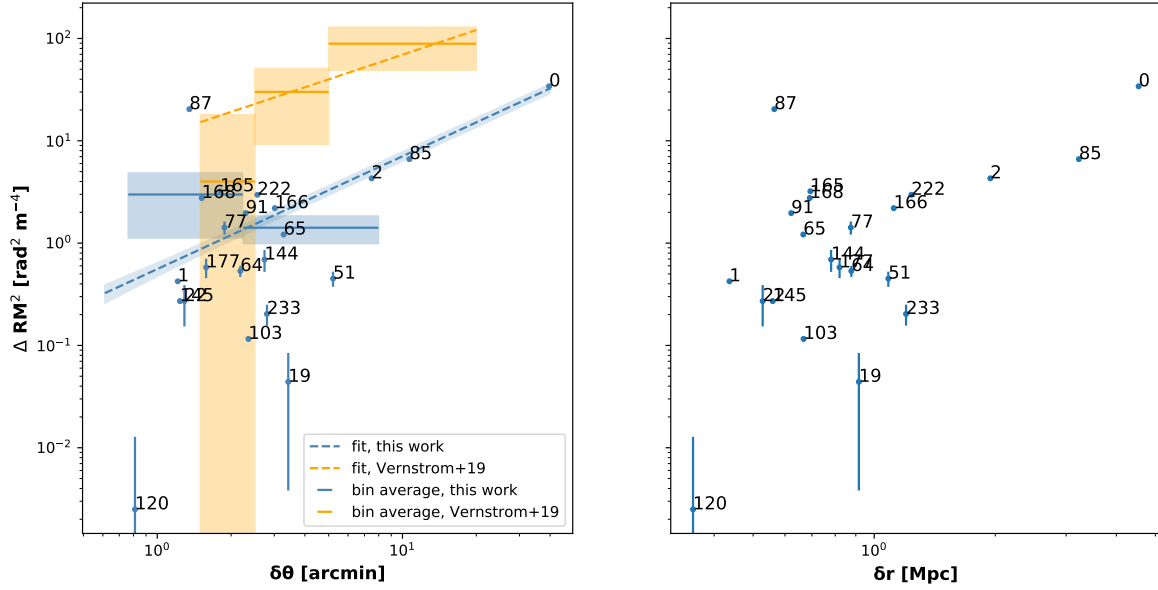
Fig. 5. Squared RM difference versus angular ( left ) and physical ( right ) separation between the detected lobes. A number corresponds to each GRG and the numbers are listed in Table 2. The blue dashed line is the power-law fit to the data with 1\sigma uncertainty (see Sect. 3.1). Orange bars show the binned averages between 1.5' and 20' obtained by Vernstrom et al. (2019) for physical pairs observed at 1.4 GHz and the dashed orange line shows the derived structure function. Blue bars show the binned averages of the sources in this work with an angular separation lower than 10' : Each bin contains ten sources, the uncertainty was computed as the standard deviation on the mean. Shaded areas show the uncertainties.
