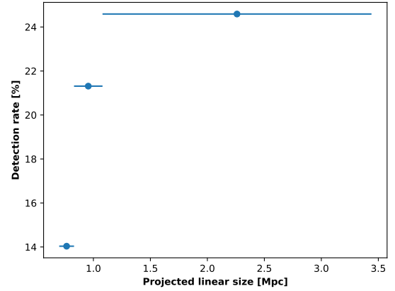
Fig. 3. Detection rate as function of the projected linear size of the GRGs from the distribution shown in the bottom panel of Fig. 2. The widths of the bins were computed to contain the same total number of sources ( \sim 60 ). The markers are positioned at the center of each bin and the error bars show the bin width.
