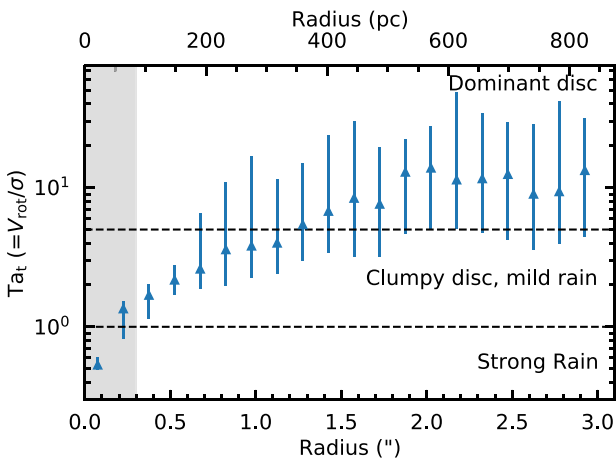
Figure 9. Median turbulent Taylor number ( Ta_t ) of the molecular gas disc in NGC 0708 (estimated within elliptical apertures and shown as blue points with error bars showing the 16th to 84th percentiles of the distribution). Formally our measurements are lower limits, due to observational effects such as beam-smearing, and hence are plotted as upward facing arrows. The central regions, where these observational effects are expected to be dominant, are shaded in grey. Dashed black horizontal lines denote the expectation for gas arising from a strong CCA rain ( Ta_t < 1 ), a mild rain (which forms a clumpy disc; 1 < Ta_t < 5 ), and a system little affected by CCA rain ( Ta_t > 5 ), as described in Gaspari et al. (2015). The central parts of NGC 0708 have a low turbulent Taylor number, consistent with bombardment by a mild CCA rain.
