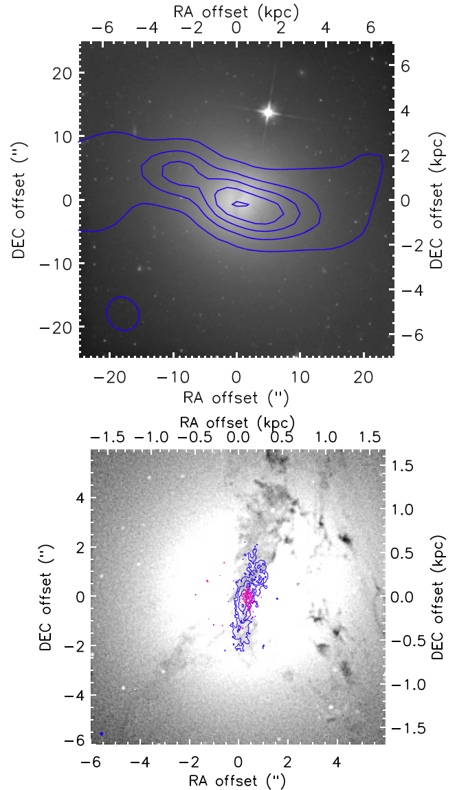
Figure 1. Top: Large-scale (50 arcsec \times 50 arcsec or \approx 14 \times 14 \text{ kpc}^2 ) HST Wide Field Camera 3 F110W image of NGC 0708, with 330 MHz continuum Very Large Array (VLA) contours from Clarke et al. (2009) overlaid in blue. Bottom: Small-scale (12 arcsec \times 12 arcsec or 3.2 \times 3.2 \text{ kpc}^2 ) HST combined Advanced Camera for Surveys and Wide Field Camera F435W image of NGC 0708, with our CO(2–1) integrated intensity ( 0''.088 or \approx 25 \text{ pc} resolution) contours overlaid in blue and 236 GHz continuum contours overlaid in magenta. The synthesized beam of the radio/millimetre data is shown in the bottom left corner of each image.
