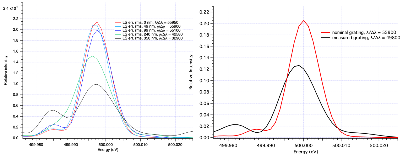
Figure 5: Simulated energy distribution after a 5 μm exit slit for the 300 l/mm grating. The simulation is performed considering an ideal grating (red curves) or with increasing rms pitch error on the grooves. RIGHT: Simulation of the expected performance of the same grating at the same energy, using the measured groove placing error.
