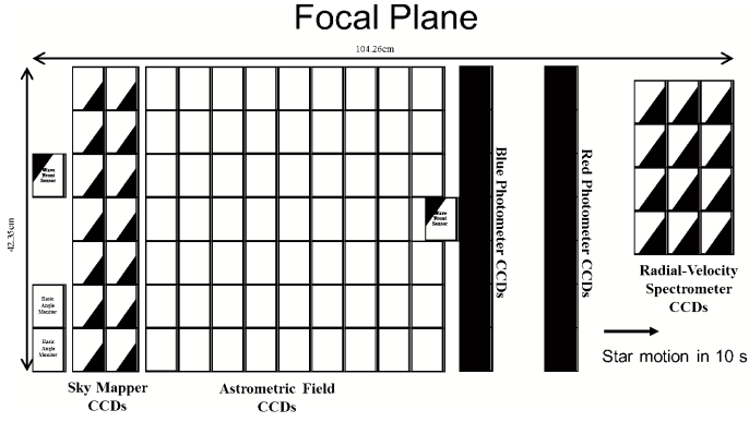
Fig. 1. Gaia focal plane, which contains 106 CCDs organised in seven rows. Stellar images travel in the along-scan direction from left to right . The 12 CCDs in green are part of the Radial Velocity Spectrometer, which will not be described any further because it is not relevant for this paper.
