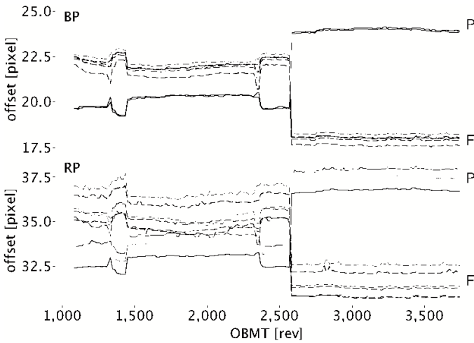
Fig. 6. Evolution in time of the geometric calibration, relative to the nominal geometry, evaluated at the centre of the CCD in the across-scan direction and for different CCDs (BP in the top panel , RP in the bottom panel ; rows from 1 to 7 are shown in red, orange, yellow, green, blue, purple, and pink). The preceding FoV is shown with brighter colours and solid lines, while darker shades and dashed lines are used for the following FoV, as indicated by the labels P and F in the plot area.
