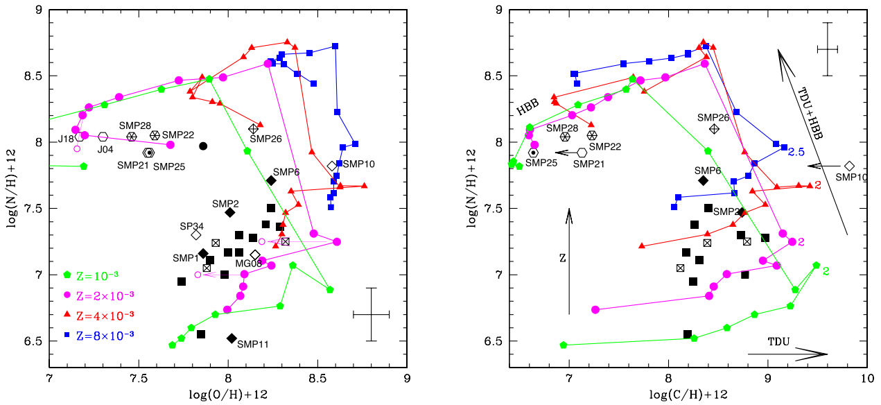
Figure 2. The observed chemical composition of the SMC PNe sample in the O–N (left-hand panel) and C–N (right) planes. Squares, hexagons, and diamonds indicate the loci of PNe, respectively, of groups (a), (b), and (c) [see Section 5]. Filled symbols mark PNe with traces of carbon dust, open-dotted symbols indicate evidence of silicates, open symbols indicate PNe with no indication of dust in the literature, and crossed symbols indicate featureless IRS spectra. We indicate the PN names for groups (b) and (c) PNe. Typical errors associated with the determination of the abundances of the individual species are indicated with crosses in the right, bottom side of the left-hand panel and in the right, top region of the right-hand panel. The final abundances of the AGB models of metallicity Z = 10^{-3} (green pentagons), Z = 2 \times 10^{-3} (magenta circles), Z = 4 \times 10^{-3} (red triangles), and Z = 8 \times 10^{-3} (blue squares) are also shown (see legend in the O–N plot). Open, magenta circles in the left-hand panel refer to Z = 2 \times 10^{-3} models calculated with a lower initial oxygen ( [O/Fe] = -0.2 ).
