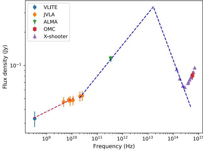
Figure 2. Jet emission between radio and optical bands, as reconstructed from VLITE, JVL A, ALMA, and X-shooter observations. The blue dashed line is a broken power law, used to identify the synchrotron peak frequency and flux density. The red line is a power-law fit of the most expanded region of the jet, considered as a physically separated component. The optical flux from OMC is also shown, although not considered for the fit.
