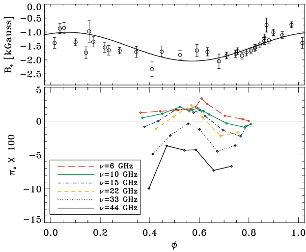
Figure 4. Bottom panel: fraction of the circularly polarized emission ( \pi_c = \text{Stokes } V / \text{Stokes } I ) as a function of stellar rotational phase. The light curves of \pi_c were calculated for each observing frequency. Top panel: effective magnetic field curve, as displayed in the top panel of Fig. 1, shown here for reference.
