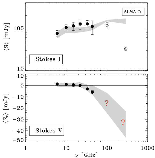
Figure 11. Results of the simulations performed increasing the magnetic field strength and changing the dipole axis orientation at \nu \leq 22 GHz. Top panel: comparison between the observed and simulated average spectrum of HR 5907 for the total intensity (Stokes I ). Bottom panel: comparison between the observed and simulated average spectrum for the circularly polarized emission (Stokes V ). The measurements at the same frequency were averaged and represented by the filled dots. These data have been already displayed in Fig. 2. The grey areas locate the range of the simulated values, constrained to the rotational phases covered by the observations.
