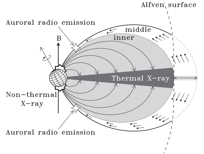
Figure B1. Magnetosphere of a dipole-shaped early-type magnetic star. The amplitude of the misalignment of the dipole and rotation axis is arbitrary. The small vectors in the middle magnetosphere-oriented towards the star represent the streams of non-thermal electrons.
