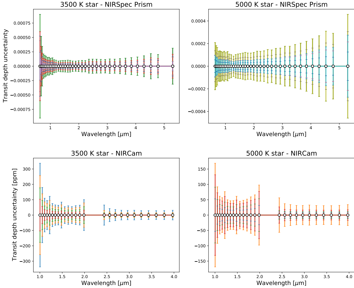
Figure 2. Transmission spectra uncertainties computed for the NIRSpect/Prism ( top ) and NIRCам/F150W2 + F322W2 ( bottom ) configurations. Increasingly larger uncertainties correspond, for NIRSpect, to mag K = 10.5, 11.5, 12.5, 13.5 and 14.5 ; for NIRCам, they correspond to K = 4.5, 6.0, 7.5 and 9.0 . M and K star scenarios are shown on the left and right column, respectively.
