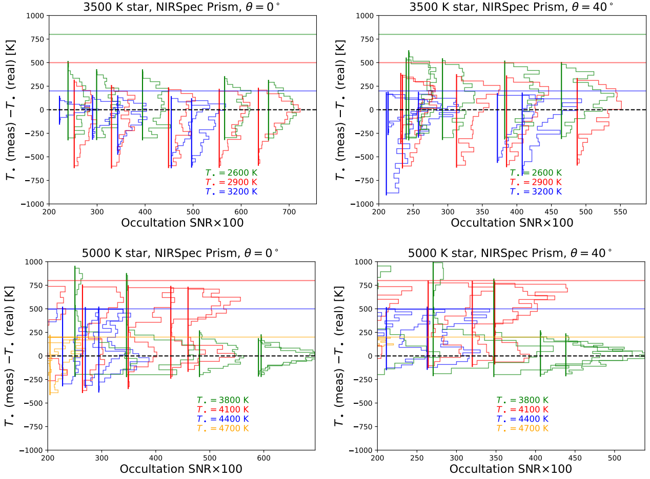
Figure B1. Posterior distributions of the difference between the measured and the true T_\star for the simulations carried out for NIRSpec/Prism, as a function of the occultation SNR multiplied for visualisation purposes. The Figures are divided by stellar temperature (rows) and starspot limb-angle (column). The baseline of each horizontal histogram indicates the SNR of the corresponding scenario and the probability in the distributions increases along the x-axis (different probability values in a given histogram are all related to the same SNR value). Different colours represent different true T_\star cases, and stellar T_\star - 100 K values (the lowest allowed in our T_\star fit) are marked with horizontal lines with the corresponding colour for each scenario. Bimodal distributions for the K star, 4100 K starspot, mid- to low-SNR case can be clearly distinguished; in the lowest SNR cases, only a lower limit can be assigned to T_\star .
