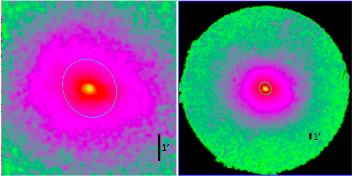
Figure 4. The X-ray surface brightness maps (0.5-2 keV) of NGC 1550 made with the Chandra (left) and XMM (right) observations. The detected point sources were removed and filled with the photons from the surrounding area (see Section 3.1.2), and the exposure correction was applied. The cyan ellipse indicates the D 25 ellipse (semi-major axis = 1 arcmin or 17 kpc) in both images.
