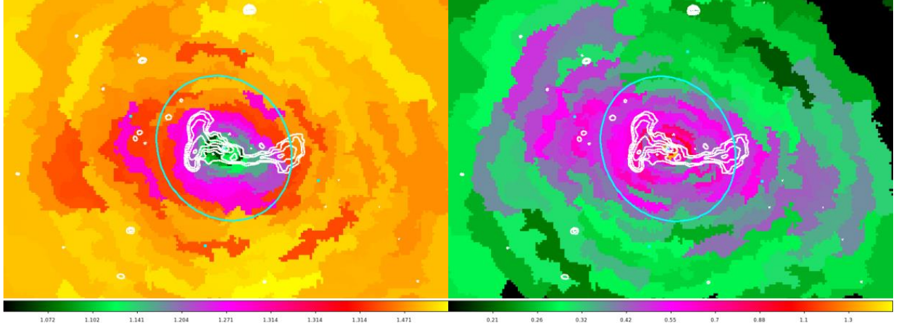
Figure 6. GMRT 610 MHz radio contours (from Kolokythas et al. 2020) showing the AGN jets and lobes are overlaid on the T map (left) and the Fe map (right). The cyan ellipse indicates the D 25 ellipse.
