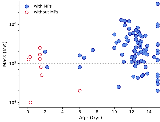
Fig. 32 Present-day mass vs. age diagram of surveyed Galactic GCs and massive clusters in the Magellanic Clouds, with and without photometrically detected MPs. A reference mass equal to 10^5 M_{\odot} is marked (see text for details).
