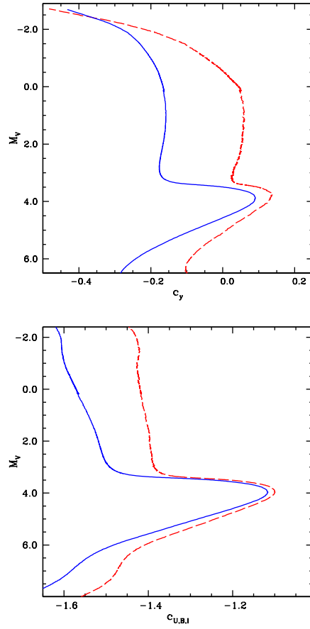
Fig. 18 Top panel: A pair of 12 Gyr, [\text{Fe}/\text{H}]=-1.6 , Y=0.246 isochrones, for both the P1 (solid line) and P2 (dashed line) compositions of Sect. 2, displayed in the M_V - c_y diagram (see text for details). Bottom panel: As the top panel, but for the M_V - c_{U,B,I} diagram (see text for details).
