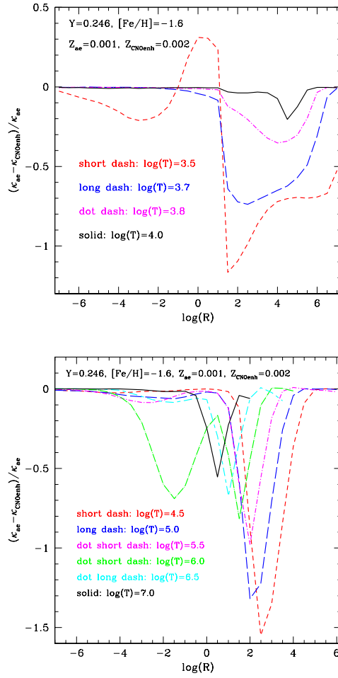
Fig. 2 Relative difference of the radiative Rosseland mean opacity between a standard P1 \alpha -enhanced composition, and the CNO-enhanced P2 CNO enh composition at fixed [\text{Fe}/\text{H}] and Y , and several temperatures (see labels), as a function of the density parameter R (see text for details). The corresponding total metal mass fractions Z are also labelled.
