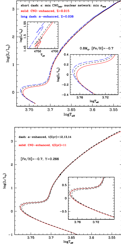
Fig. 3 Upper panel: HRD of evolutionary tracks for a 0.8M_{\odot} model computed with the \alpha -enhanced P1 composition, and the P2 \text{CNO}_{\text{enh}} metal mixture, both with the same [\text{Fe}/\text{H}] ( [\text{Fe}/\text{H}]=-0.7 ) and initial He abundance ( Y=0.266 ). The short-dashed line shows a track calculated with radiative opacities appropriate for the P2 composition, but the same CNO abundances of the P1 composition in the nuclear burning network (see text for details). The two insets show the RGB bump and the TO-SGB regions, respectively. Lower panel: HRD of theoretical isochrones computed with the same P1 and P2 compositions of the upper panel, and various ages. The inset shows the TO-SGB regions.
