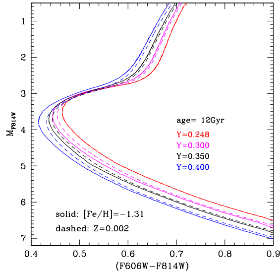
Fig. 27 Optical CMD from the MS to the lower RGB in the ACS filter system, for 12 Gyr isochrones with the various labelled initial values of Y and either constant [\text{Fe}/\text{H}] or constant Z .
