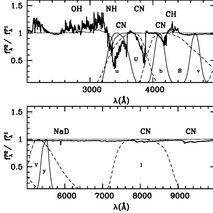
Fig. 13 Top panel: Ratio of the fluxes calculated from P1 and P2 RGB model atmospheres with T_{\text{eff}}=4,500 K, surface gravity \log(g)=2 (cgs units – thick solid line) and TO model atmospheres with T_{\text{eff}}=6,131 K, \log(g)=4.5 (thin solid line), respectively. The wavelength range between 2000 and 5000 Å is displayed, together with the transmission curves of the U and B Johnson filters, plus the u , b , and v Strömgen filters. The labelled molecules mainly contribute to the absorption in those wavelength ranges where P1 and P2 results are different. Bottom panel: As the top panel, but for the wavelength range between 5,000 and 10,000 Å, and the transmission curves of the V and I Johnson-Cousins filters, and the y Strömgen filter.
