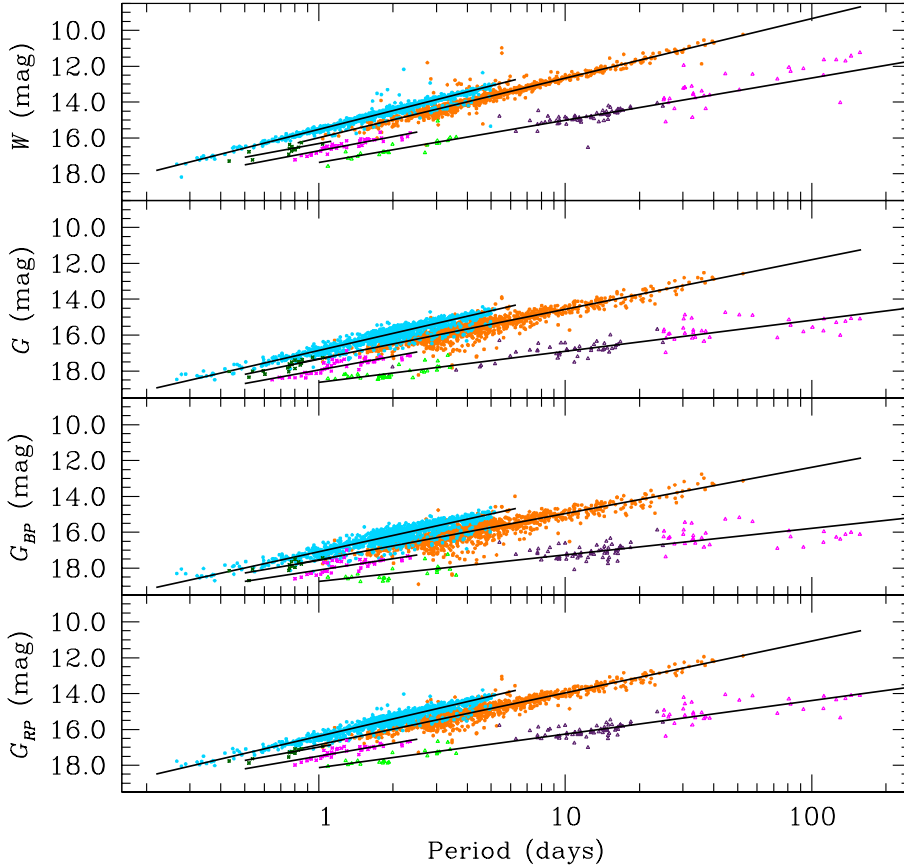
Fig. 1. For the LMC, PL/PW relations in the form mag = \alpha + \beta \log P . From top to bottom panels, mag is represented by the apparent W , G , G BP , and G RP magnitudes, respectively. Orange filled circles: DCEP_F; cyan filled circles: DCEP_10; magenta four-starred symbols: ACEP_F; dark green four-starred symbols: ACEP_10; green open triangles: BLHER; violet open triangles: WVIR; and magenta open triangles: RVTAU.
