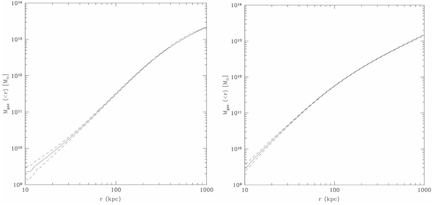
Figure 4. Enclosed gas mass M_{\text{g}}(<r) profiles for A2465 NE (left) and SW (right). Dashed curves indicate 1\sigma or 68% confidence levels.
