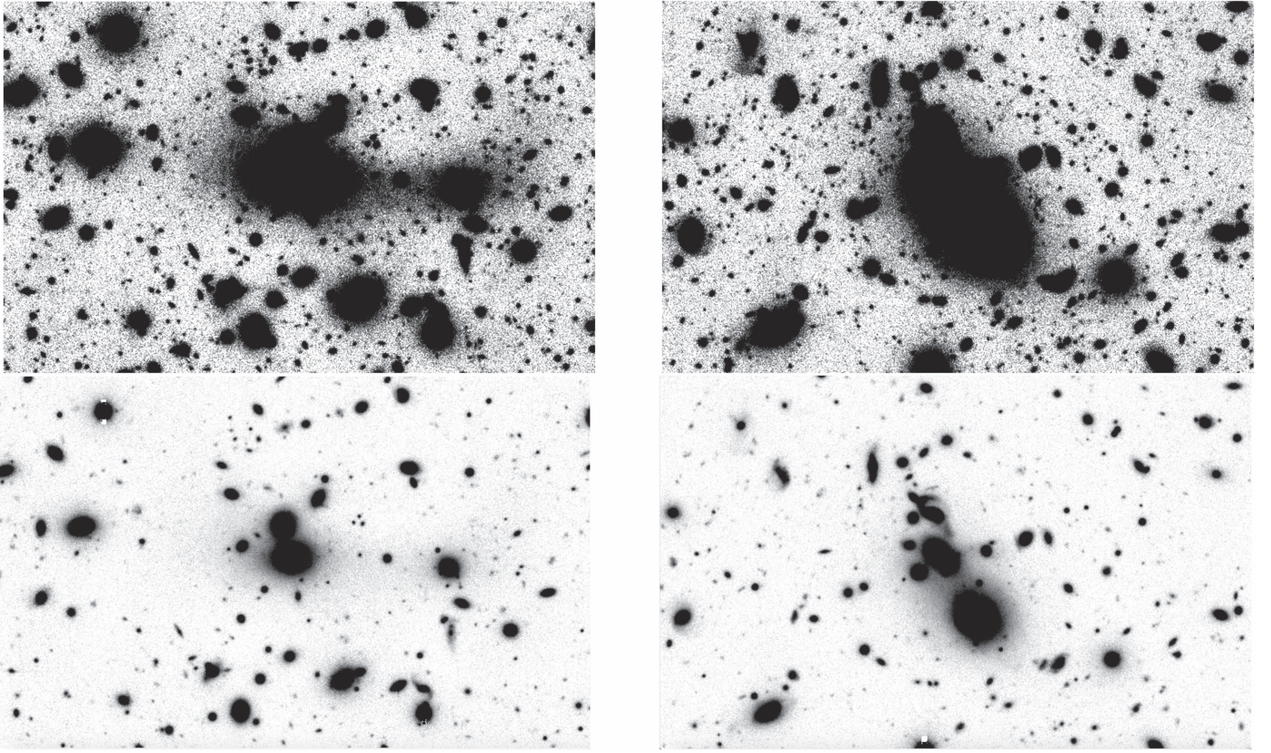
Figure 2. Centers of the subcomponents of A2465 from the combined Suprime-Cam Viz' images described in Section 3 showing the BCGs. The NE (left) component and the SW (right) component are shown. North is to the top and west to the right. The vertical edge of each image is about 1.5 arcmin or 345 kpc. The top row shows faint details near the sky limit. The bottom row brings out the peaks of the brightest objects.
