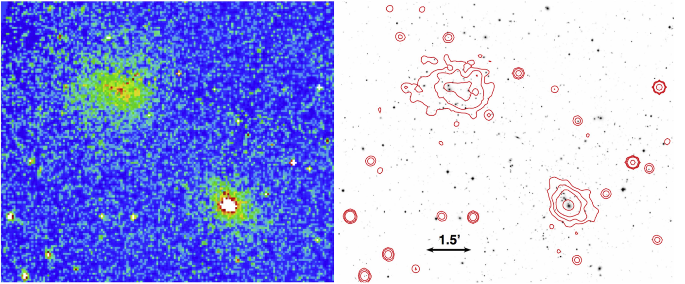
Figure 1. Left: Chandra image of A2465 in the 0.5 to 3.0 keV energy band with 8 pixel binning. Right: CFHT megaprime i' image with the isodensity X-ray contours. North is to the top and west to the right. The images are approximately 11 \times 9 arcmin 2 . The NE component is to the upper left and comparison with the SW component shows the differences in their structures. The X-ray center of the NE subcluster is slightly displaced from its central BCGs while the SW X-ray peak is nearly centered on the BCG.
