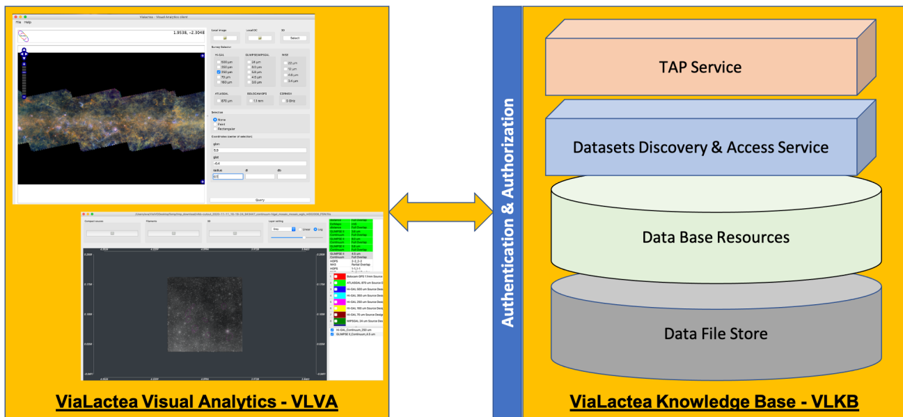
Figure 1. ViaLactea Visual Analytics (VLVA) application interacting with the ViaLactea Knowledge Base (VLKB) exposing the contained file store and metadata through the TAP service and the datasets discovery & access service
