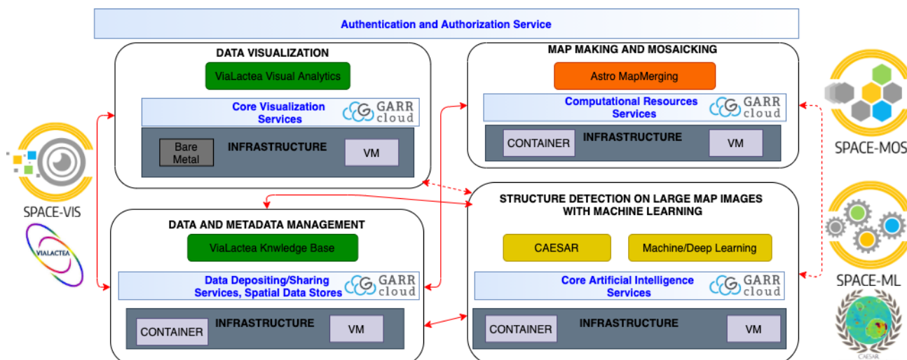
Figure 2. NEANIAS Visual Analytics Services delivery and integration with core services.
