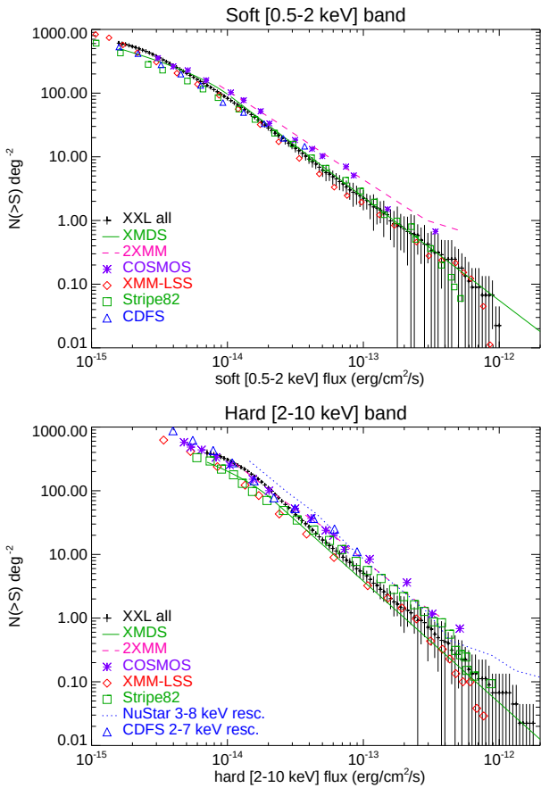
Fig. 4. \log N - \log S relation for both XXL areas in the soft and hard X-ray bands (black crosses with 1\sigma error bars), compared with some literature measurements (see text for details).
