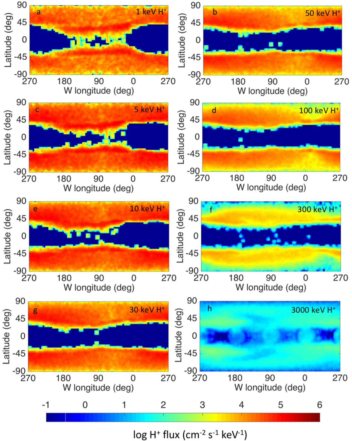
Figure 3. H^+ precipitation maps in science case (ii) (Ganymede is near the center of JPS) corresponding to different initial energies. Smaller granular structures in regions where the flux is very low (e.g., the equator) are caused by the finite number of test particles. The W longitude system has been used meaning the leading hemisphere is at long \sim 90^\circ and long \sim 0^\circ is at the Jupiter-facing hemisphere apex.
