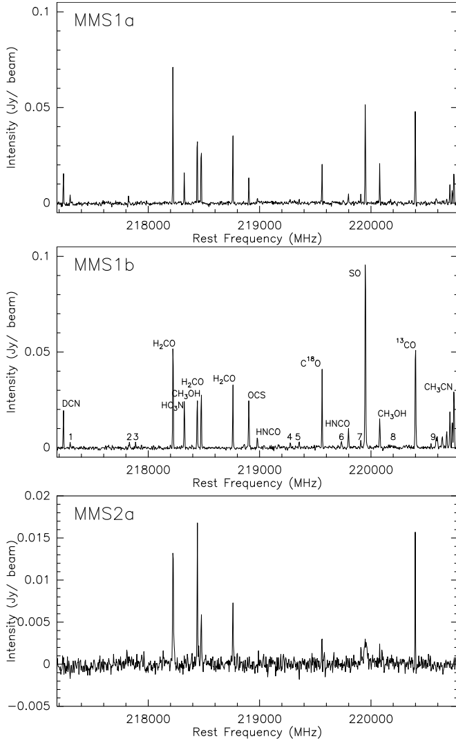
Fig. 2. Spectra towards the three major cores from the broadband correlator unit data obtained from averaging the central 0.5'' around the continuum emission peak. The spectral resolution in these bands is \sim 2.7 \text{ km s}^{-1} or \sim 1.95 \text{ MHz} . The molecule labels are given for the chemically rich core MMS1b. We note that the flux scale is smaller for MMS2a. Lines labeled with numbers are: (1) and (3) unidentified, (2) ^{33}\text{SO} , (4) \text{SO}_2 , (5) ^{34}\text{SO}_2 , (6) and (9) \text{HNCO} , (7) \text{H}_2^{13}\text{CO} and (8) \text{CH}_2\text{CO} .
