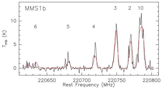
Fig. 7. Spectrum of the \text{CH}_3\text{CN} ( 12_K-11_K , K = 0-6 ) transitions towards the continuum emission peak in MMS1b. The red curve indicates the best fit as obtained from the XCLASS procedures, with T_{\text{rot}} = 85\text{ K} and N_{\text{H}_2} = 5.4 \times 10^{14}\text{ cm}^{-2} .
