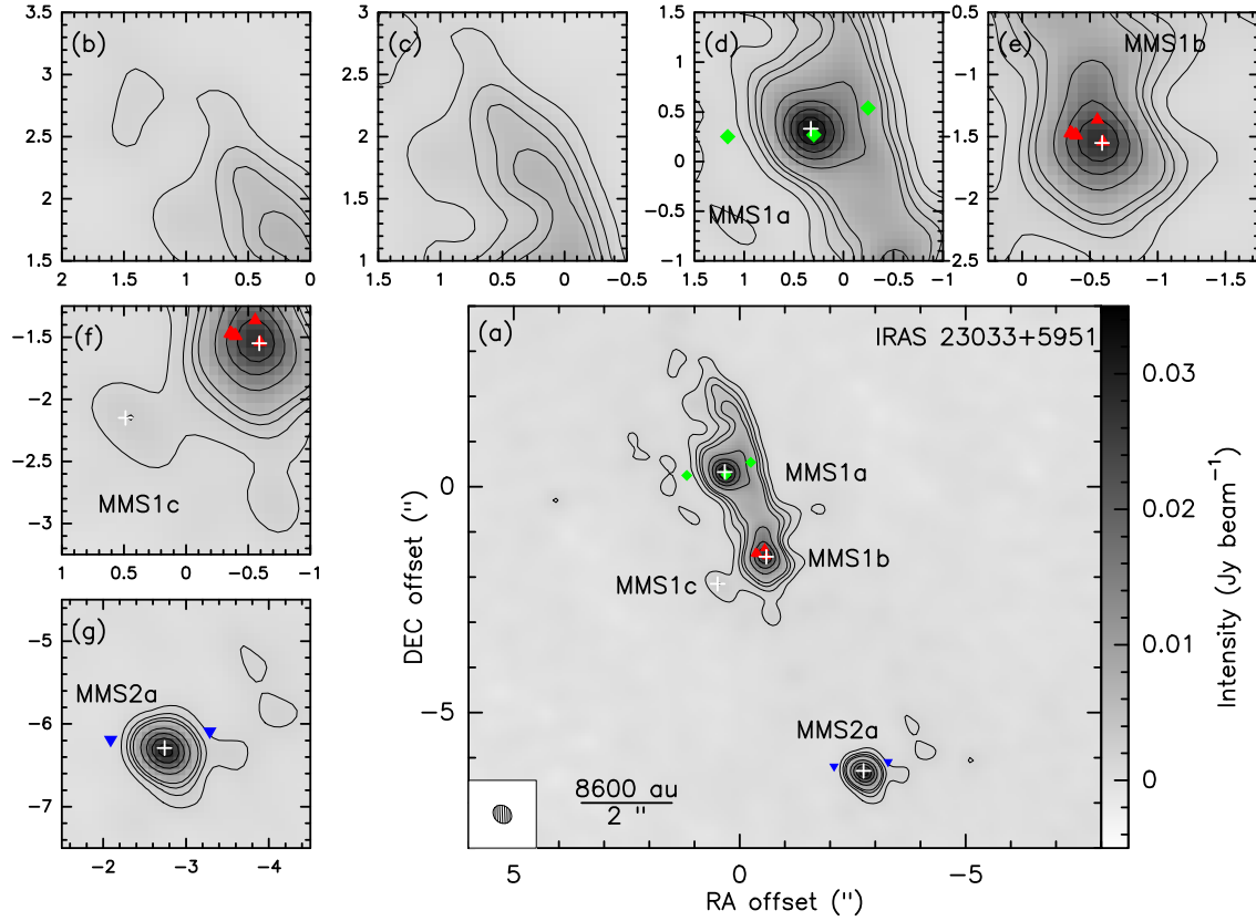
Fig. 1. Continuum emission towards IRAS 23033+5951 at 1.37 mm, with a phase center at RA 23^{\text{h}} 05^{\text{m}} 25^{\text{s}}.00 and Dec +60^{\circ} 08' 15''.49 (J2000.0). The black contours indicate the 5, 10, 15, 20\sigma levels and increase further in steps of 20\sigma , where \sigma = 0.28 \text{ mJy beam}^{-1} . The corresponding negative values are absent in the presented region. The white + and labels mark the mm sources identified by CLUMPFIND. The green, red, and blue symbols are cm point sources, \text{H}_2\text{O} masers (both Rodríguez et al. 2012), and methanol masers (Rodríguez-Garza et al. 2017), respectively. The shaded ellipse in the bottom left shows the synthesized beam of 0.45'' \times 0.37'' (PA 47^\circ ). The small panels zoom in on the elongation of the core MMS1a (b,c), MMS1a (d), MMS1b (e), MMS1c (f) and MMS2a (g).
