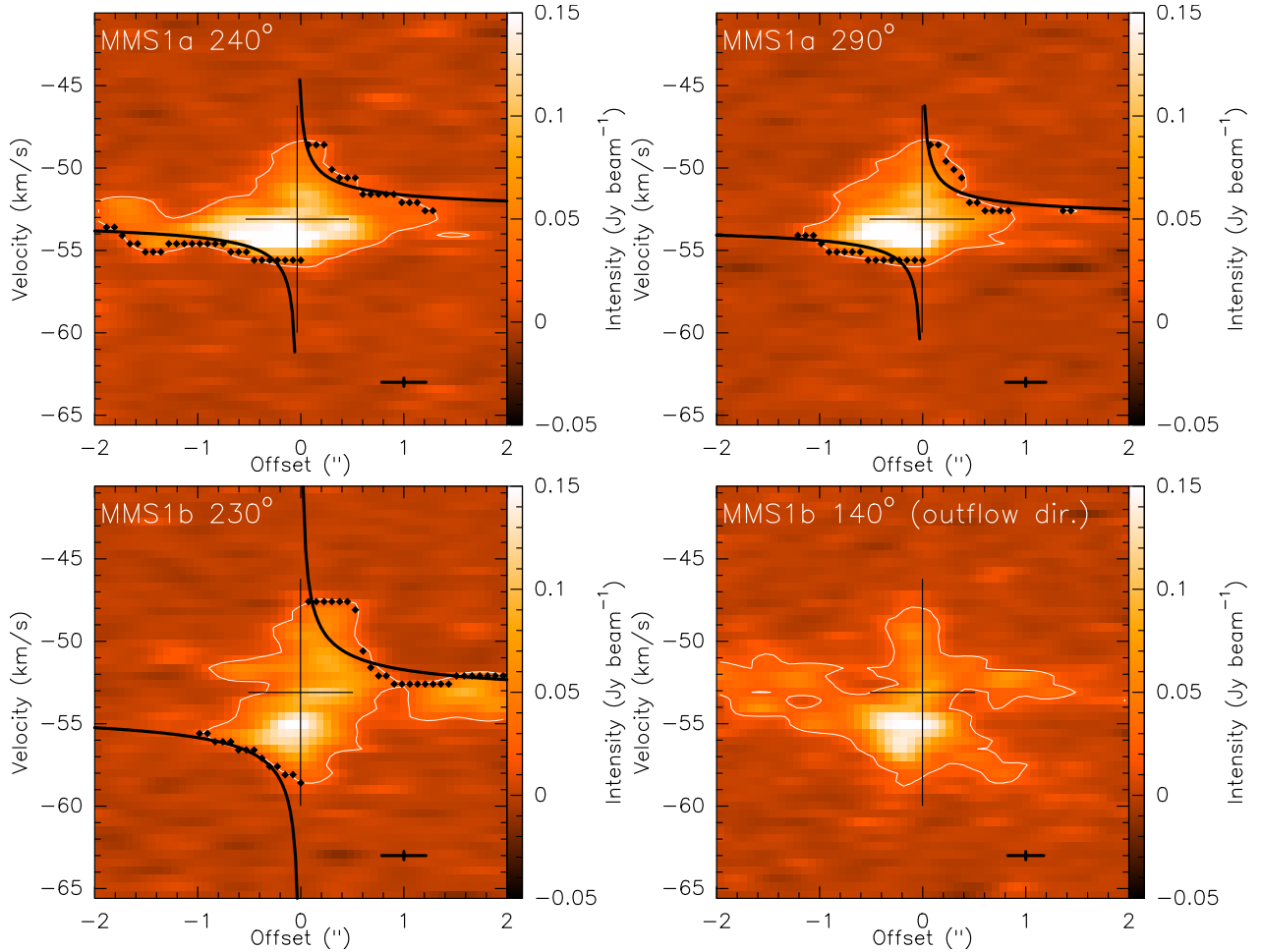
Fig. 9. Position–velocity diagrams for the \text{H}_2\text{CO} ( 3_{0,3}-2_{0,2} ) transition towards the two major cores MMS1a and b from the NOEMA data, with a synthesized beam of \approx 0.43'' \times 0.35'' (PA 61^\circ ). The cut directions are shown in Fig. 8. The bottom right PV diagram is from a cut through MMS1b, perpendicular to the left cut and along the inferred outflow axis (see Sect. 3.4). The white contour shows the 4\sigma detection threshold. The black vertical and horizontal bars indicate the position of the continuum emission peak and the systemic velocity, respectively. Their lengths correspond to 1'' \approx 4300 \text{ au} and 14 \text{ km s}^{-1} . The black dots indicate the detection with the most extreme velocity at each position. The black solid curves indicate the Keplerian velocities, corresponding to the mass estimates in Table 4. The black crosses in the lower right corners indicate the resolution elements along both axes.
