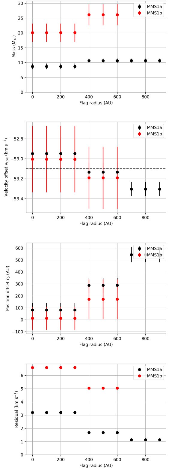
Fig. A.2. Best-fit results for the tests of flagging the inner region around the YSO. The routine was applied to the PV diagrams from the \text{H}_2\text{CO} ( 3_{0,3}-2_{0,2} ) image. The error bars are the standard deviations from the least-squares fits. The horizontal line in the velocity plot is the systemic velocity of the source IRAS 23033+5951.
