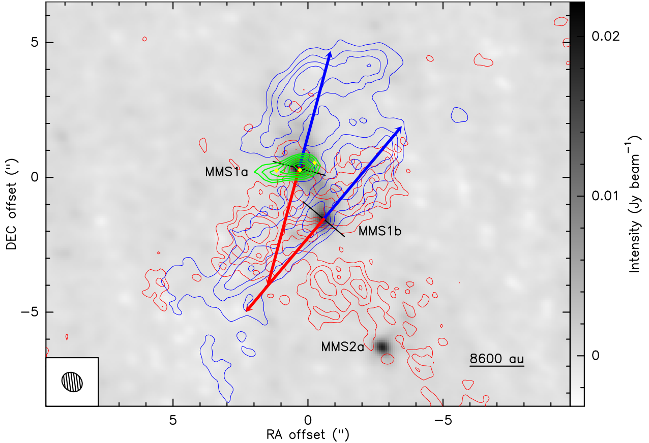
Fig. 6. Multiple outflow structures towards IRAS 23033+5951 as traced by ^{13}\text{CO} (2–1) emission in the merged data cube. The gray-scale in the background shows the continuum intensity from Fig. 1. The blue and red contours present the integrated line wing emission from ^{13}\text{CO} for the intervals of -70 to -60\text{ km s}^{-1} and -46 to -36\text{ km s}^{-1} ( v_{\text{LSR}} = -53.1\text{ km s}^{-1} ), respectively, starting at 55% and increasing in steps of 10% of the peak intensities I_{\text{peak,blue}} = 0.78\text{ Jy beam}^{-1}\text{ km s}^{-1} and I_{\text{peak,red}} = 0.25\text{ Jy beam}^{-1}\text{ km s}^{-1} . The green contours show the continuum emission at 3.6 cm, reported by Beuther et al. (2002a), starting at 4\sigma and increasing in steps of \sigma = 41.5\text{ }\mu\text{Jy beam}^{-1} with an angular resolution of 1.04'' \times 0.62'' , and the yellow diamonds towards MMS1a mark the positions of the 3.6 cm emission peaks (Rodríguez et al. 2012) with an angular resolution of 0.31'' \times 0.25'' . The blue and red arrows are drawn by eye to guide the reader to the outflow lobes from MMS1a and b. The solid lines across the cores are drawn perpendicular and indicate the corresponding inferred disk major axes. The shaded ellipse in the lower left corner indicates the synthesized beam of 0.8'' \times 0.67'' (PA 52^\circ ) of the merged ^{13}\text{CO} (2–1) data.
