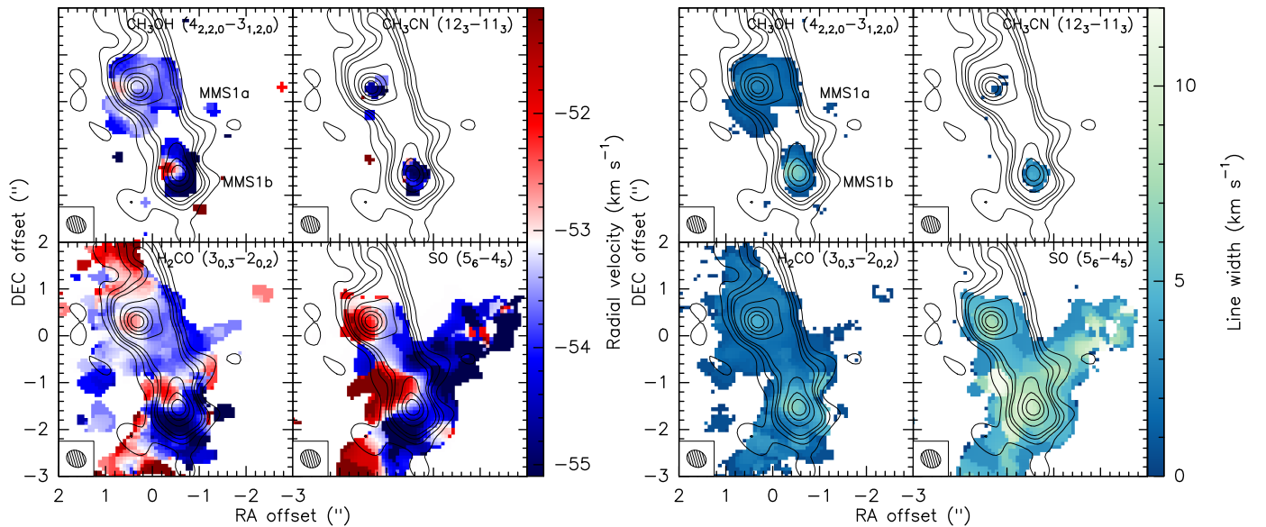
Fig. 4. Spectral line emission towards IRAS 23033+5951. For the first (intensity-weighted peak velocity, left panels ) and second-order moment maps (line width, right panels ), the flux was integrated over the velocity range v_{\text{LSR}} \pm 10 \text{ km s}^{-1} , with v_{\text{LSR}} = -53.1 \text{ km s}^{-1} , considering emission above the 5\sigma threshold of each respective molecule. The black contours indicate the 5, 10, 15, 20\sigma continuum emission levels and increase further in steps of 20\sigma , where \sigma = 0.28 \text{ mJy beam}^{-1} . The dashed ellipses in the lower left corner of each panel show the respective synthesized beam \approx 0.43'' \times 0.35'' (PA 61^\circ ).
