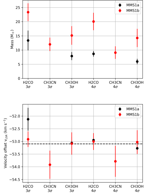
Fig. A.1. Best-fit estimates of kinematic mass ( top ) and systemic velocity ( bottom ) for thresholds of 3 and 4\sigma for the YSO mass and velocity ( v_{\text{LSR}} ), respectively. The error bars are the standard deviations from the least-squares fits. The horizontal line in the velocity plot is the systemic velocity of the source IRAS 23033+5951.
