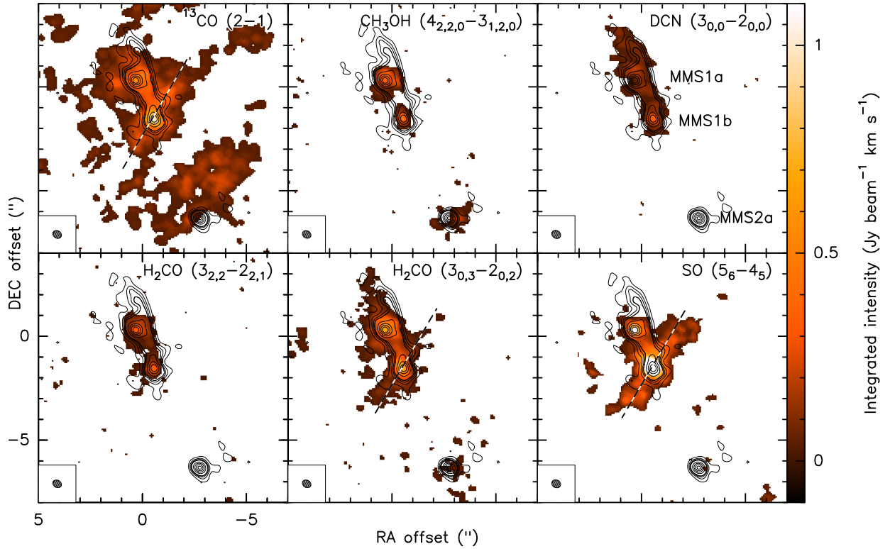
Fig. 3. Spectral line emission from selected molecular species towards IRAS 23033+5951. For the integrated intensity (zeroth order moment) maps, the intensity was integrated over the \pm 10 \text{ km s}^{-1} around the v_{\text{LSR}} = -53.1 \text{ km s}^{-1} and above the 5\sigma threshold of each respective molecule. The black contours indicate the 5, 10, 15, 20\sigma continuum emission levels and increase further in steps of 20\sigma , where \sigma = 0.28 \text{ mJy beam}^{-1} . The dashed ellipses in the lower left corner of each panel show the respective synthesized beam \approx 0.43'' \times 0.35'' (PA 61^\circ ). The dashed lines indicate an elongated structure through MMS1b.
