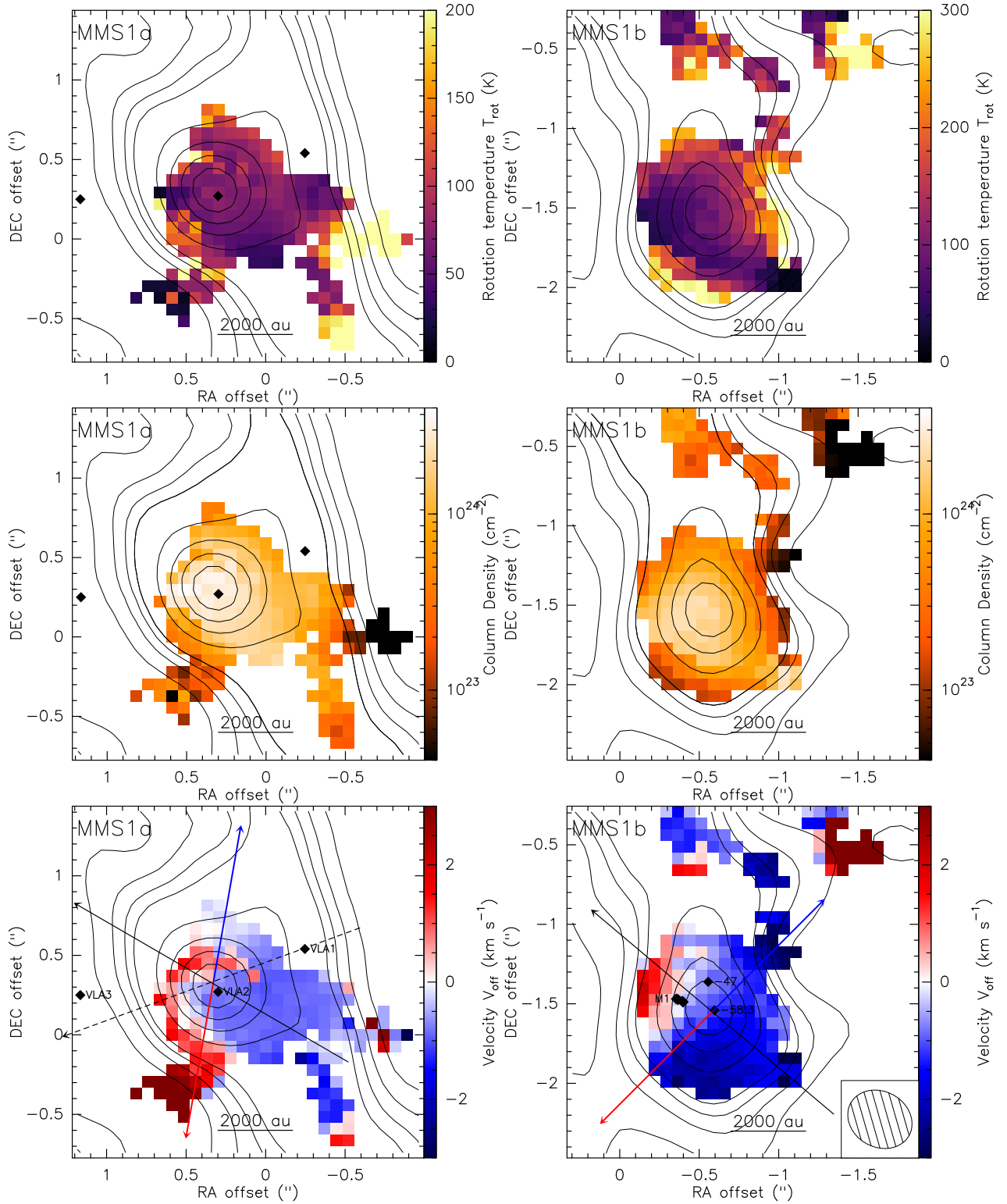
Fig. 8. Results of the radiative transfer modeling with XCLASS of the \text{CH}_3\text{CN} ( 12_K-11_K , K = 0-6 ) data. The maps cover 2.2'' \times 2.2'' extracted around the two major cores MMS1a and b, where pixels with flux below 6\sigma_{\text{CH}_3\text{CN}} were blanked out. The black contours indicate the 5, 10, 15, 20\sigma continuum emission levels and increase further in steps of 20\sigma , where \sigma = 0.28 \text{ mJy beam}^{-1} . The black diamonds in the MMS1a panel mark the positions of the emission peaks at 3.6 cm (Rodríguez et al. 2012). The shaded ellipse in the lower right corner indicates the synthesized beam of the \text{CH}_3\text{CN} data of 0.42'' \times 0.35'' (PA 61^\circ ). Details to the spectral line map fit are summarized in Sect. 3.5. Top : rotational temperature maps from XCLASS. Middle : \text{H}_2 column density maps, estimated from the continuum intensity I_\nu (Fig. 1), and rotational temperature T_{\text{rot}} (top panels) using Eq. (2). Bottom : velocity offsets from XCLASS. The colors indicate the relative velocity with respect to the v_{\text{LSR}} = -53.1 \text{ km s}^{-1} . In the MMS1b panel, the additional black diamonds mark the positions of the \text{H}_2\text{O} masers with the corresponding velocity in \text{km s}^{-1} from Rodríguez et al. (2012). The M1 maser group contains maser emission with velocities ranging from -37.2 to -66.8 \text{ km s}^{-1} . The blue and red arrows are the outflow axes as in Fig. 6. The solid and dashed black arrows are the cut directions for the PV diagrams presented in Fig. 9, along the presumable disk semi-major axes.
