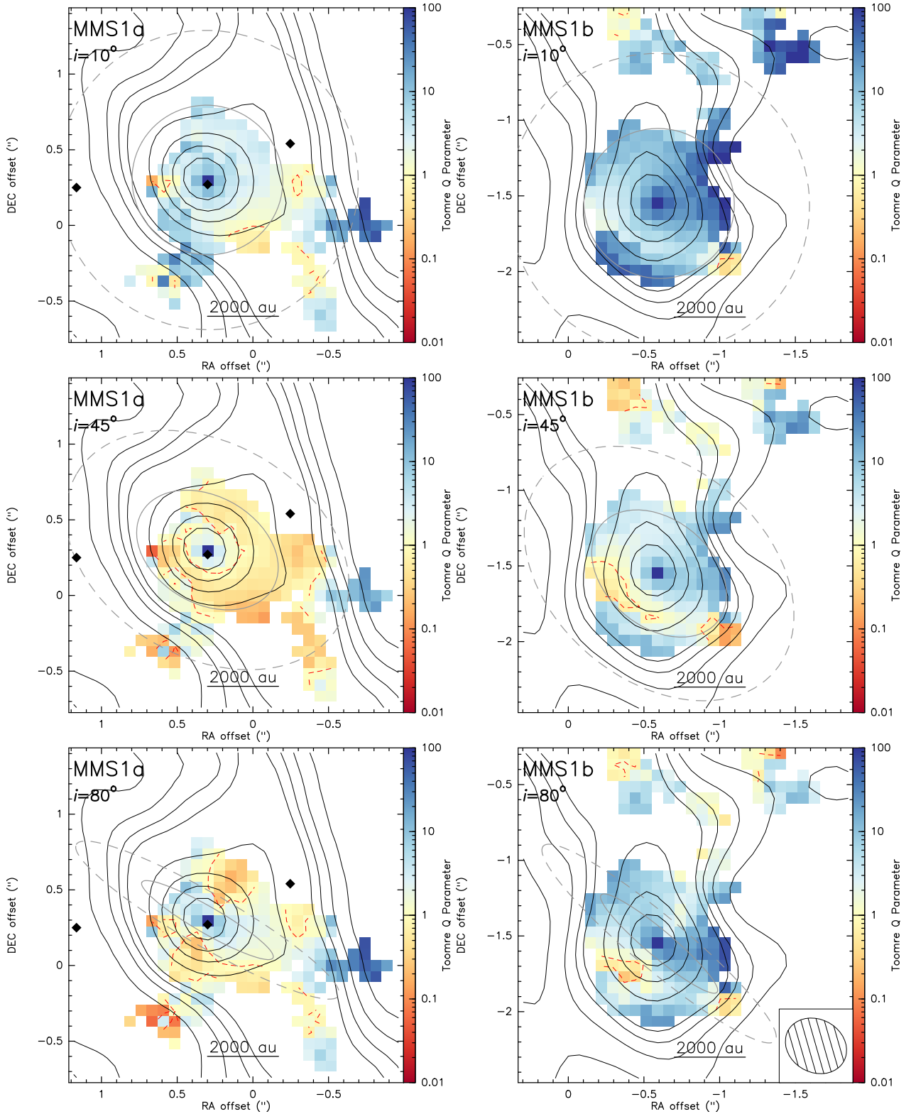
Fig. 11. Maps of Toomre's Q parameter towards MMS1a and b. The color scale indicates the value of Toomre's Q parameter, where blue is Toomre-stable, yellow is critical, and red regions are gravitationally unstable against axisymmetric perturbations, where the level of Q_{\text{crit}} = 1 is indicated by the red dashed contours. The black contours indicate the 5, 10, 15, 20 \sigma continuum emission levels and increase further in steps of 20 \sigma , where \sigma = 0.28 \text{ mJy beam}^{-1} . The solid and dashed gray ellipses show the deprojected radii of the disks with diameter 4300 and 8600 au, respectively. The black diamonds in the MMS1a panels mark the positions of the emission peaks at 3.6 cm (Rodríguez et al. 2012). Top panels: Q parameter maps of the two cores for the rotating disk structures seen almost face-on ( i = 10^\circ ). Motivated by the disk inclination estimate of i_{\text{MMS1b}} \sim 80^\circ (Rodríguez et al. 2012), we also present maps for such disk inclinations ( bottom panels ) and intermediate values ( i = 45^\circ , middle panels ). For the deprojection process, the angles of the disk major axes of \phi_{\text{maj,MMS1a}} \approx 240^\circ and \phi_{\text{maj,MMS1b}} \approx 230^\circ (relative to the north–south axis, see text) were used. The shaded ellipse in the lower right corner indicates the synthesized beam of the \text{CH}_3\text{CN} data of 0.42'' \times 0.35'' (PA 61^\circ ).
