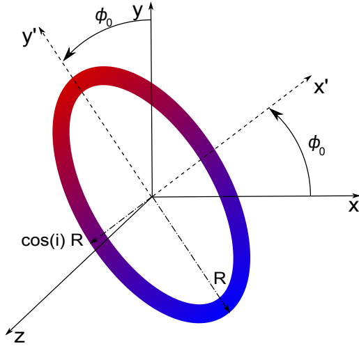
Fig. B.1. Sketch of the inclined disk ellipse model for the initialization of the map of the deprojected radius, which was used to obtain a map of the epicyclic frequency \Omega_{\text{epi}} .
