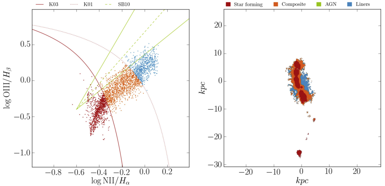
Figure 8. Left: diagnostic diagram of the ionizing sources across the galaxy. The red dotted and continuous lines are defined as in Kewley et al. (2001) and Kauffmann et al. (2003), respectively. The green lines are taken from Sharp & Bland-Hawthorn (2010; see the text for details.) Right: spatial locations of the spaxels color-coded based on the ionizing source diagnostic. H \alpha continuum surface brightness contours are shown as a reference for the stellar emission.
