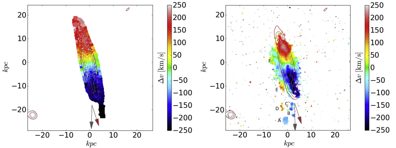
Figure 5. Left panel: stellar velocity map. Right panel: gas velocity map. The solid lines in both figures are the H\alpha continuum surface brightness contours in four logarithmically spaced levels. Regions labeled “A” to “F” are described in the text. The gray and red arrows point toward the BCG and the cluster X-ray emission, respectively. A cut of 4 in S/N was applied in the gas velocity map. North is up, east is left.
