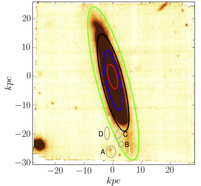
Figure 9. MUSE datacube integrated with respect to the wavelength. The ellipses are the areas where the SFR is computed, with the same color-coding as in Figure 10. The gray ellipses and circles on the southern part are the four H \alpha blobs as identified in Section 5.1.
