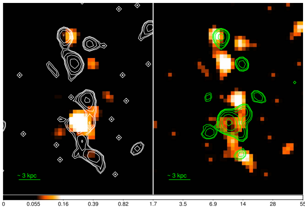
Figure 14. Chandra 2–10 keV (left) and 0.3–2 keV (right) images of the GASP cluster galaxy JO36.
